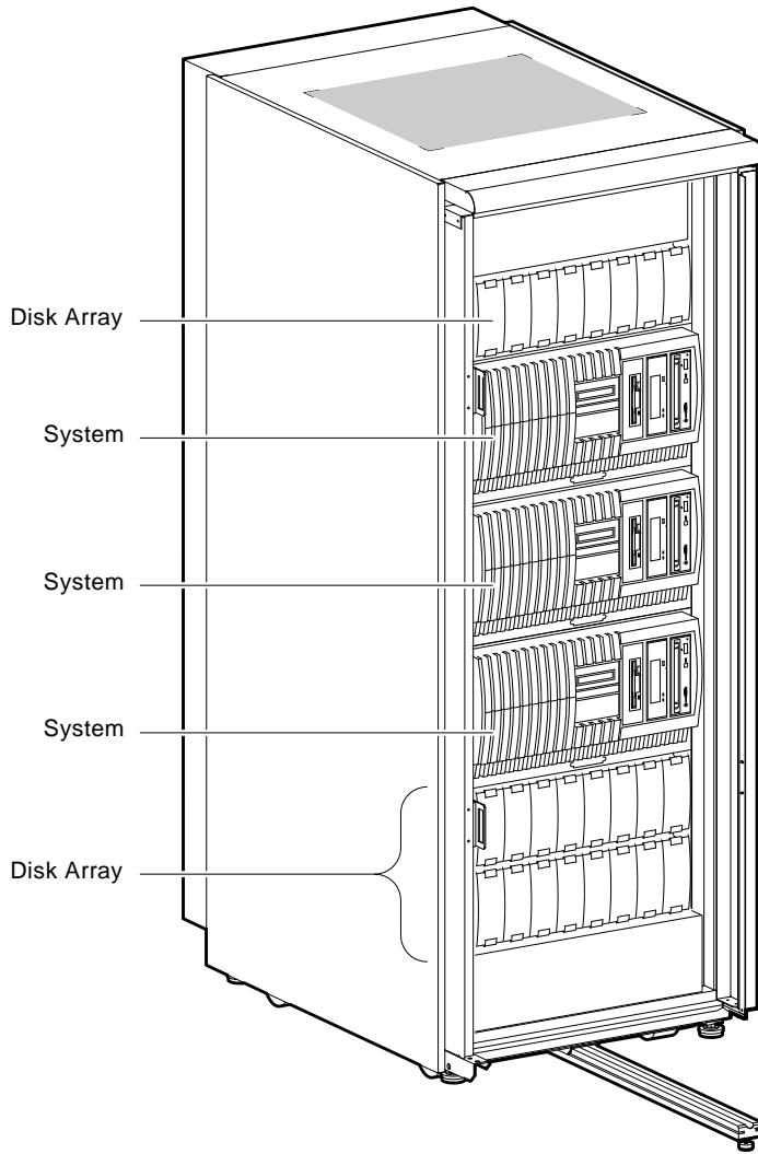
Figure 8 AlphaServer 1000 CAB System Components
