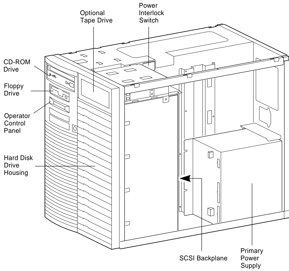
Figure 5 AlphaServer 1000 System Front View
