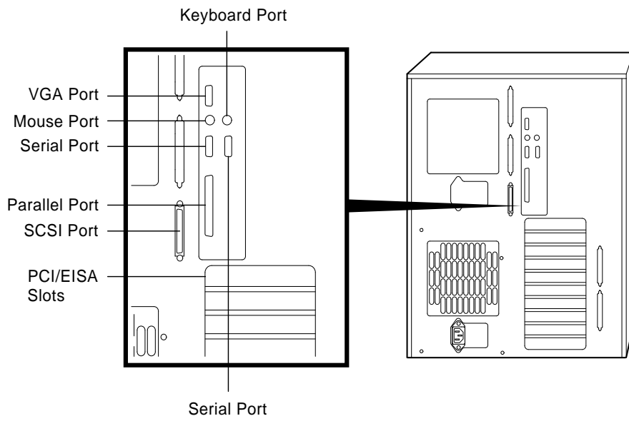
Figure 7 AlphaServer 1000 System Rear View
