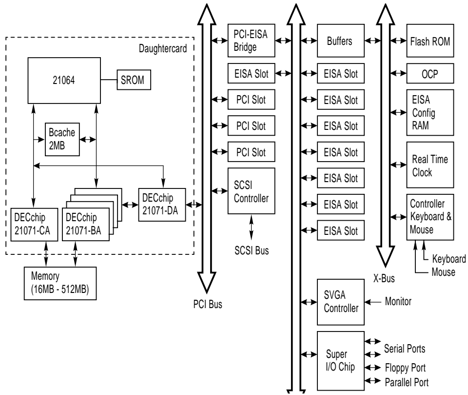
Figure 4 System Architecture
