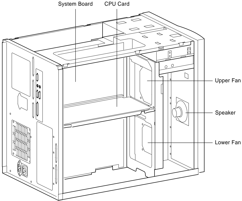
Figure 6 AlphaServer 1000 System Side View
