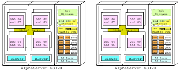
AlphaServer GS320 AlphaServer GS320
