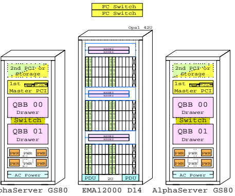
AlphaServer GS80 EMA12000 D14 AlphaServer GS80
