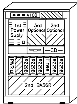
AlphaServer 4100 on the floor
