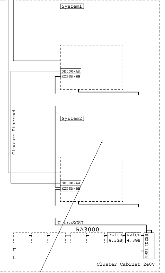
DA-AAHZA-BA/BB Ready to Go Cabinet, 120V/240V
