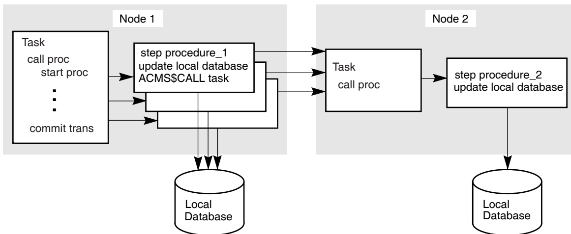
Figure 6–8 Remote Update Using Called Task from Procedure
