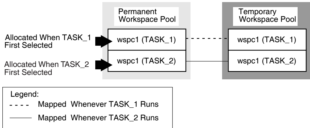
Figure 6–3 Declaring Group Workspaces in the Task Definition
