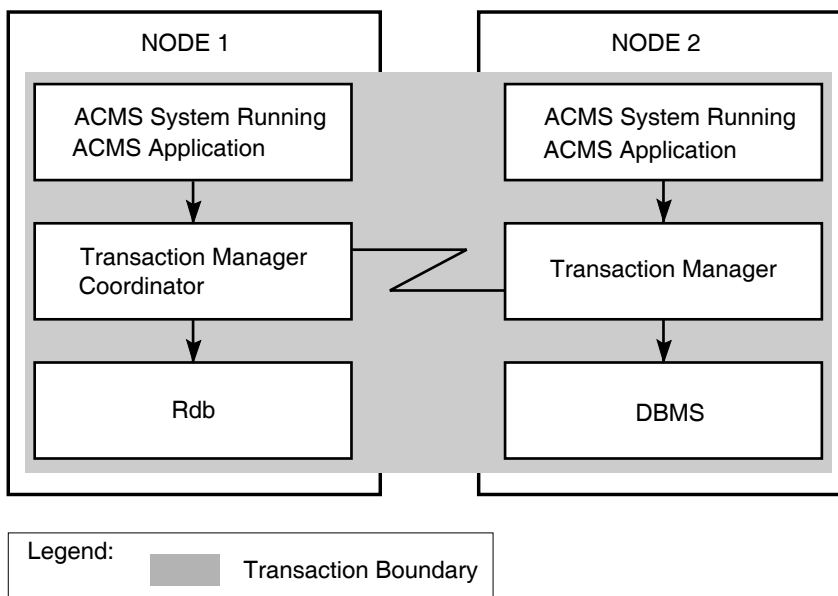
Figure 1–11 Coordinating Multiple Resource Managers
