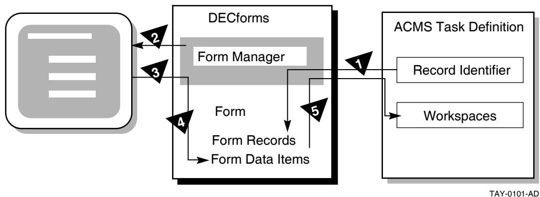
Figure 1–7 HP DECforms Interaction with ACMS
