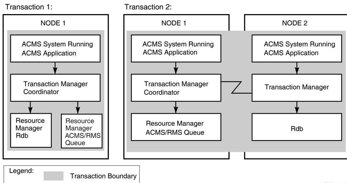
Figure 1–12 Coordinating Task Queues with Database Updates
