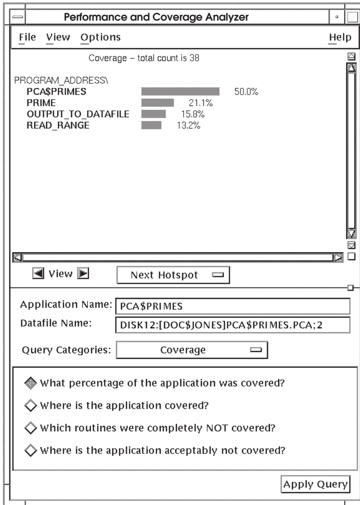
Figure 6–1 Test Coverage Histogram
