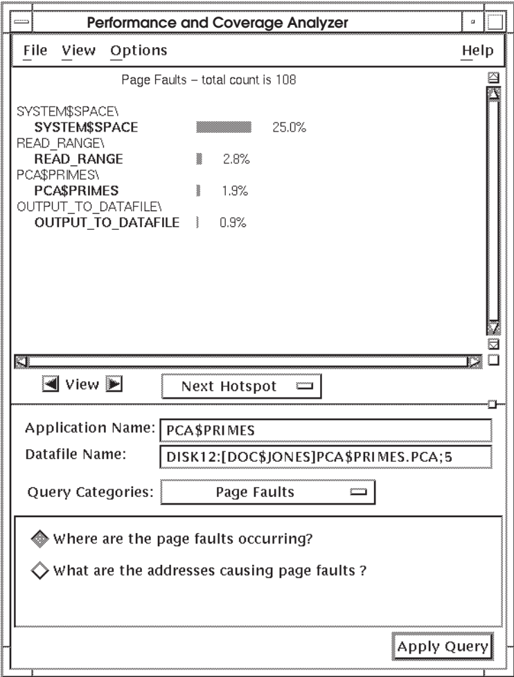
Figure 7-6 Histogram Showing Where Page Faults Are Occurring
