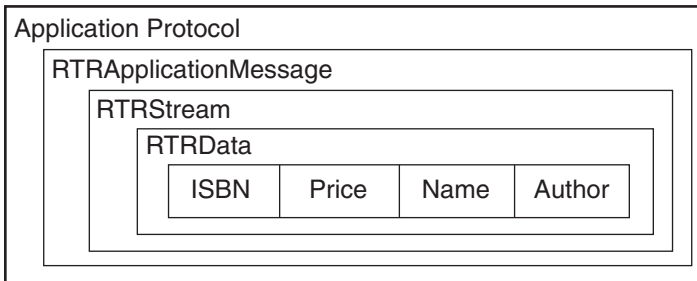
Figure 1–4 RTRData Encapsulation
