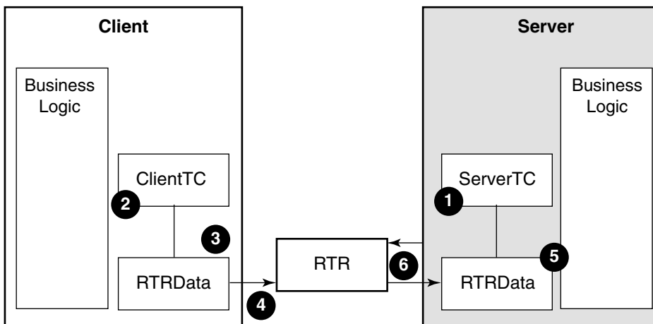
Figure 1–5 Client/Server Interaction
