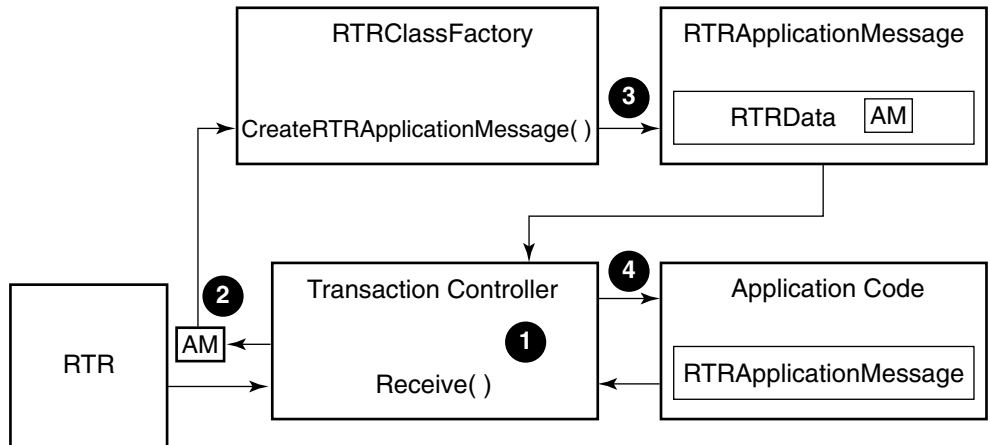
Figure 1–6 Receiving an Application Message
