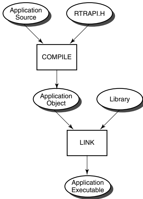
Figure 1–18 RTR Compile Sequence
