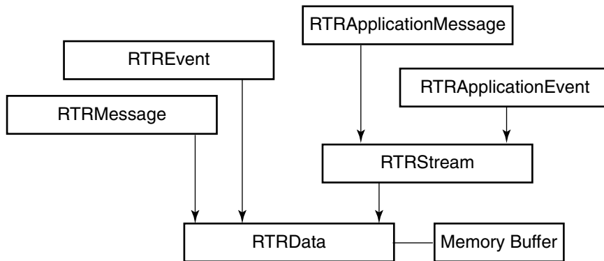
Figure 1–3 Data Classes
