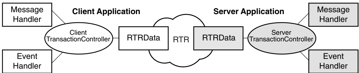
Figure 1–2 C++ API Classes
