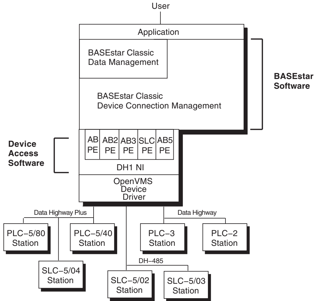
Figure 1–1 DAS Communications
