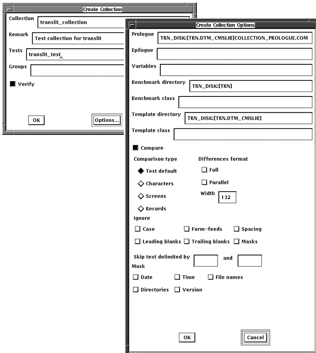
Figure 10–4 Create Collection Dialog Box
