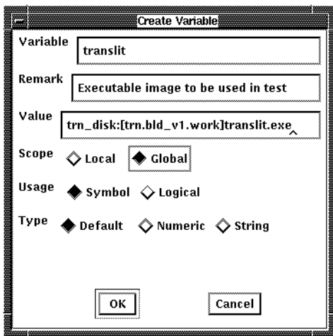
Figure 10–3 Create Variable Dialog Box
