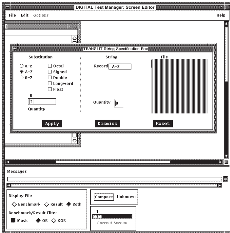
Figure 10–9 Creating a Benchmark Mask
