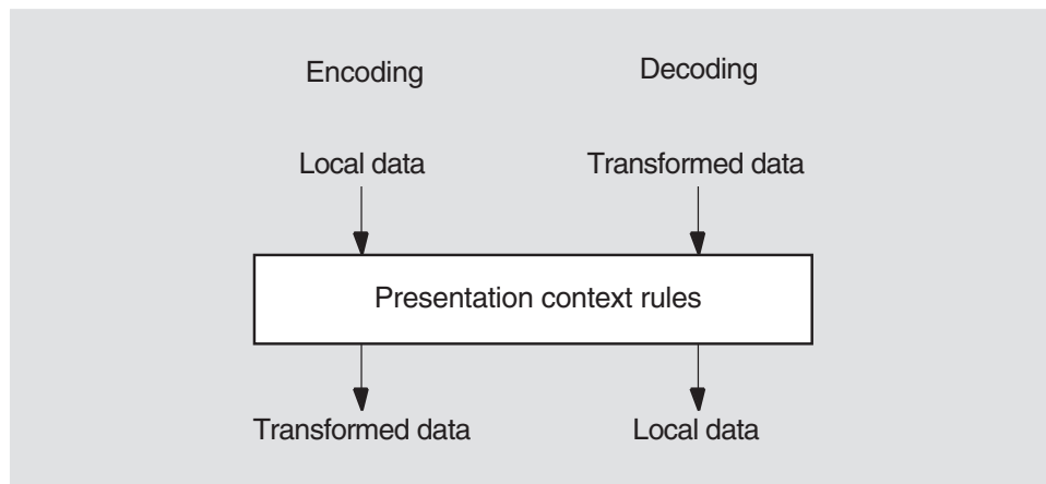
Figure 6–4 Syntax Transformation
