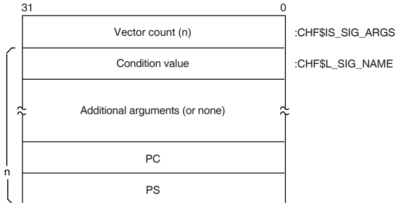
Figure 2–3 Signal Array
