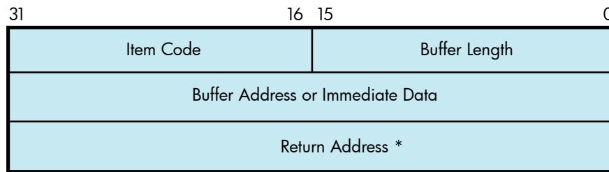
Figure 5-4 Itemlist Read Descriptor
