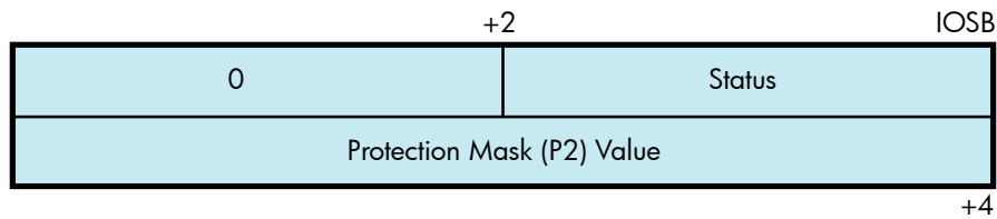
Figure 4-10 IOSB Contents— Set Protection Function
