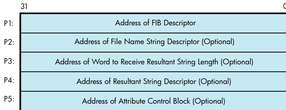
Figure 1-1 ACP Device- or Function-Dependent Arguments
