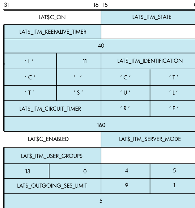
Figure 5-10 Example SETMODE Itemlist
