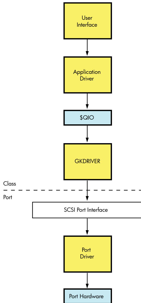
Figure 8-2 Generic SCSI Class Driver Flow
