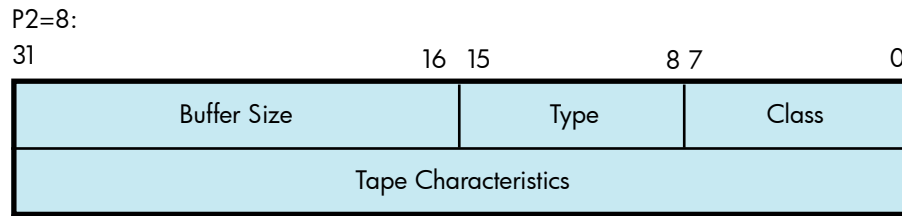
Figure 3-5 Set Mode Characteristics Buffer for IO$_SETCHAR
