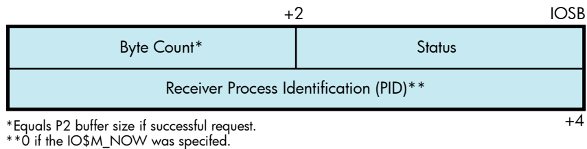
Figure 4-9 IOSB Contents— Write Function
