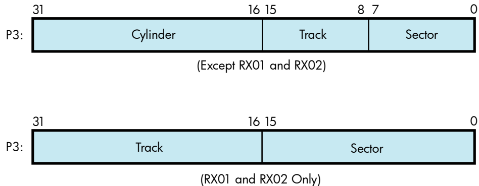
Figure 2-1 Starting Physical Address
