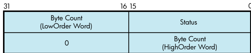
Figure 2-5 IOSB Contents
