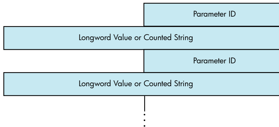
Figure 9-14 P2 Extended Characteristics Buffer
