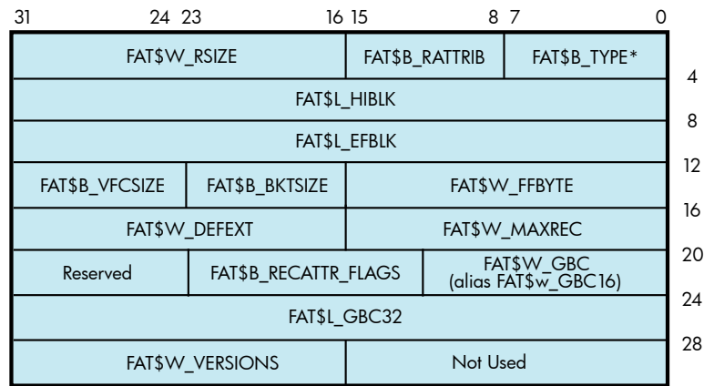
Figure 1-5 ACP-QIO Record Attributes Area
