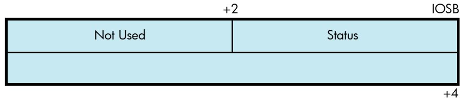
Figure 1-8 IOSB Contents — ACP-QIO Functions
