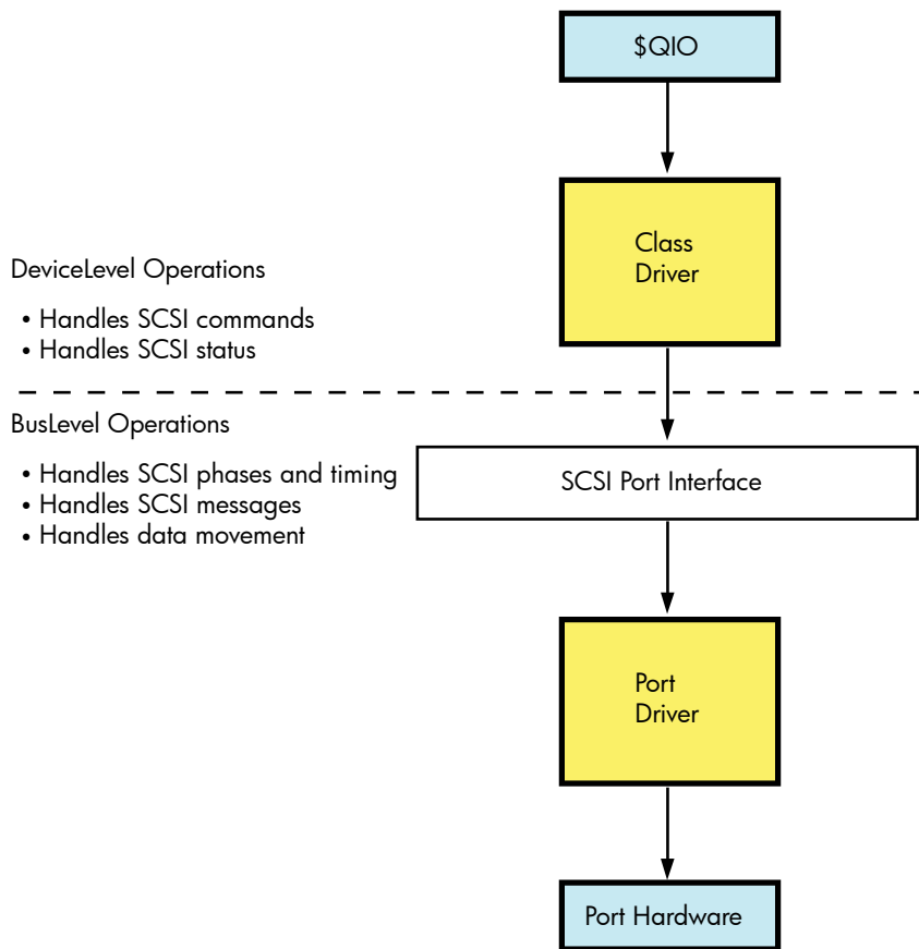
Figure 8-1 OpenVMS SCSI Class/Port Interface
