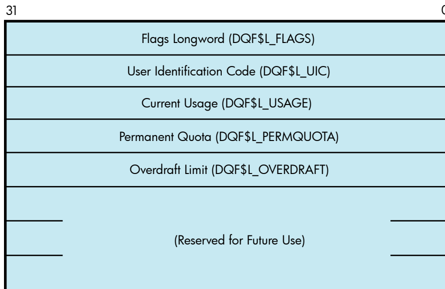
Figure 1-7 Quota File Transfer Block
