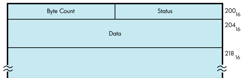
Figure 6-1 Buffer Layout
