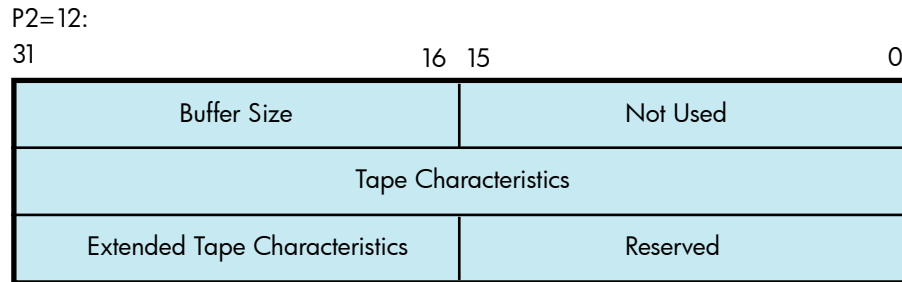
Figure 3-5 Set Mode Characteristics Buffer for IO$_SETCHAR
