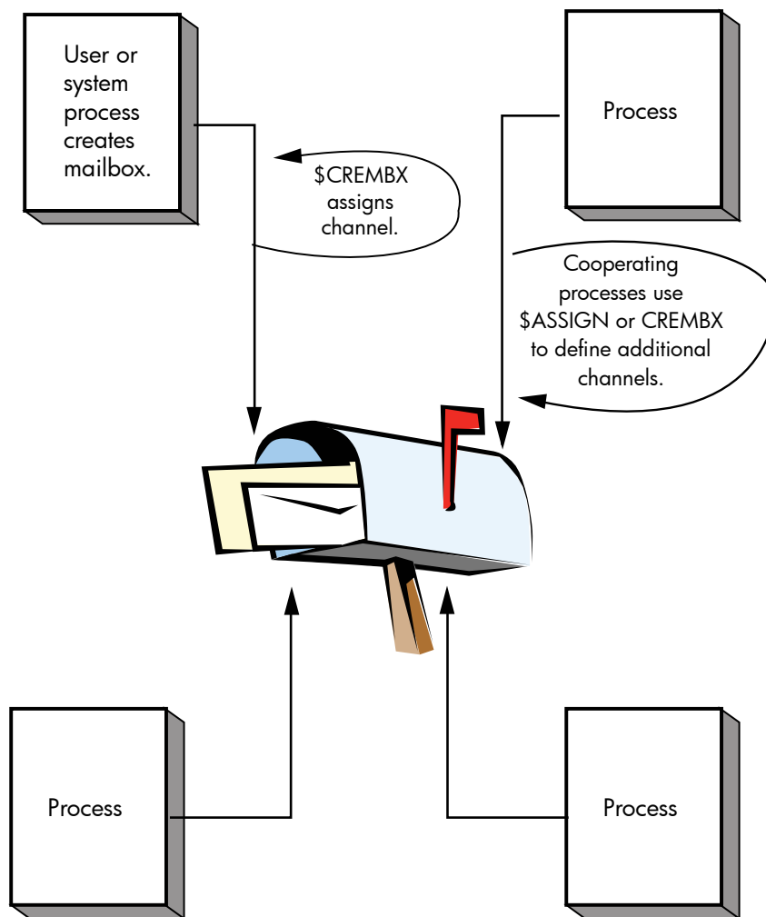
Figure 4-1 Multiple Mailbox Channels
