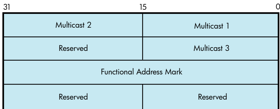
Figure 9-19 Format of IO$M_SHOW_MAP P2 Buffer
