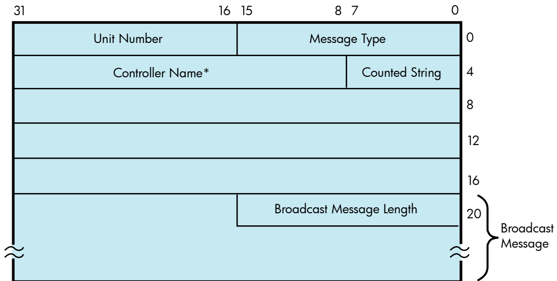
Figure 5-2 Terminal Mailbox Message Format
