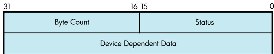
Figure 3-6 IOSB Contents
