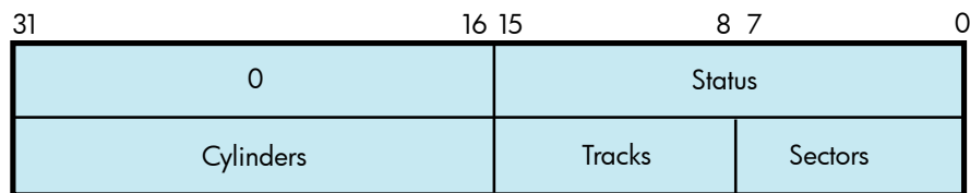
Figure 2-6 IOSB Contents for the Sense Mode Function
