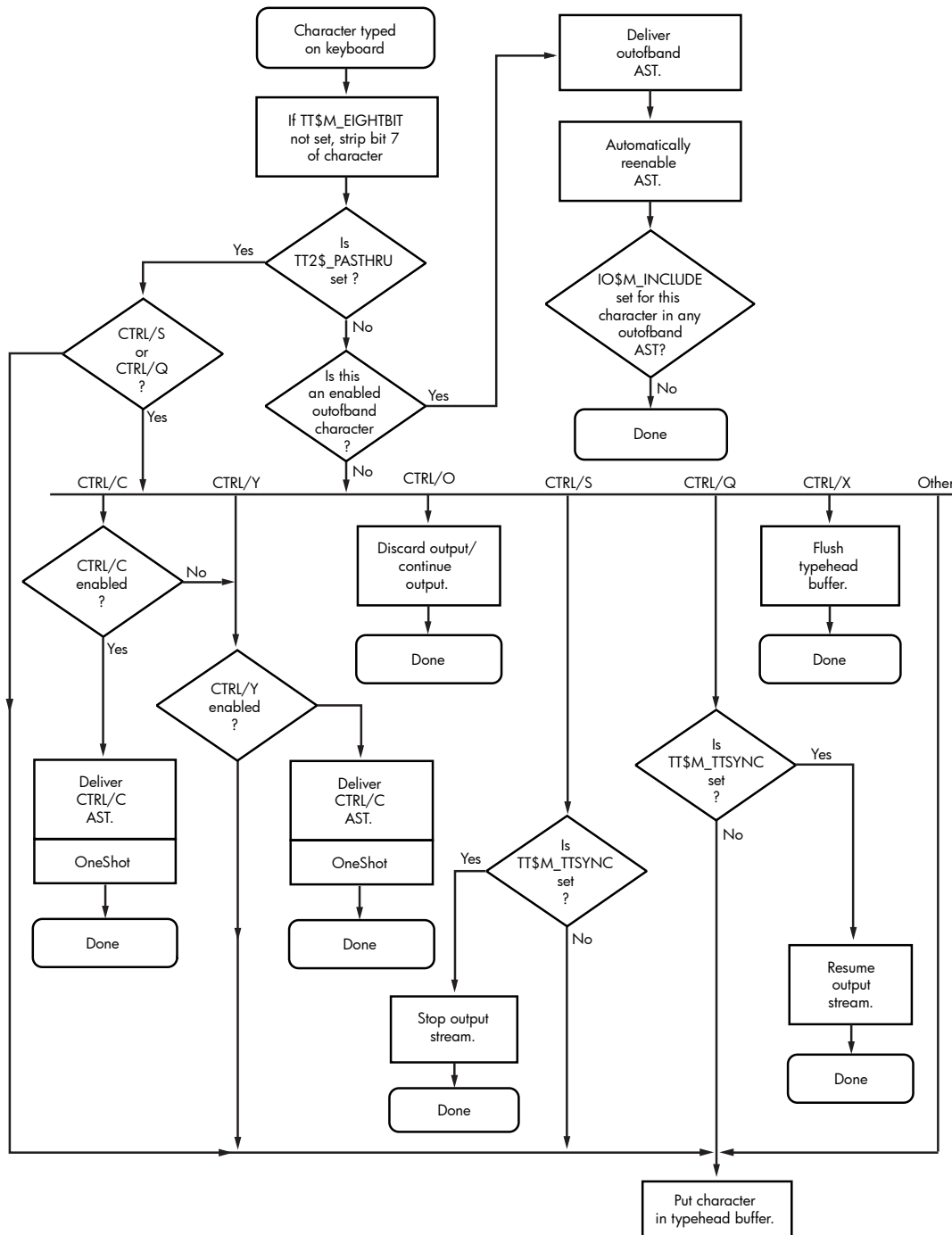
Figure 5-9 Relationship of Out-of-Band Function with Control Characters
