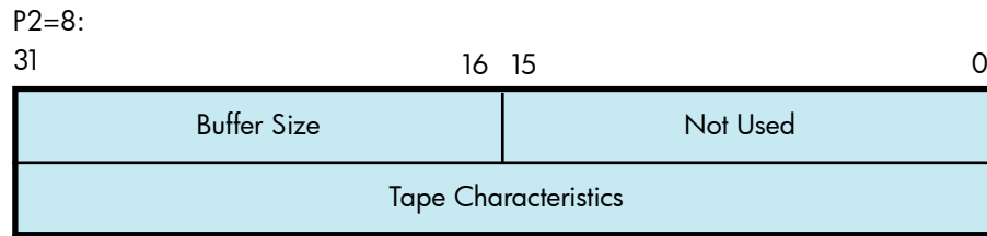
Figure 3-4 Set Mode Characteristics Buffer for IO$_SETMODE
