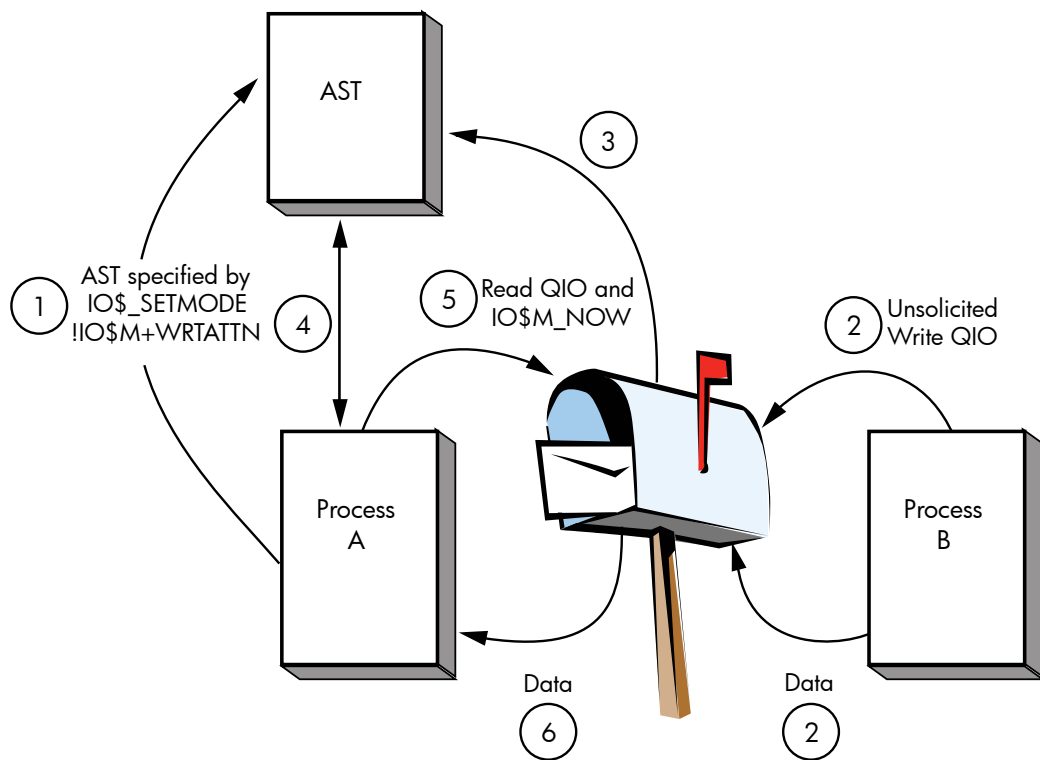
Figure 4-5 Write Attention AST (Read Unsolicited Data)
