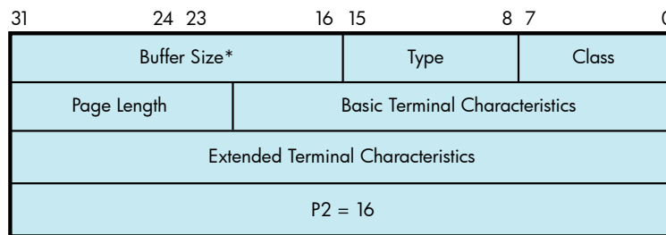
Figure 5-11 Sense Mode Characteristics Buffer
