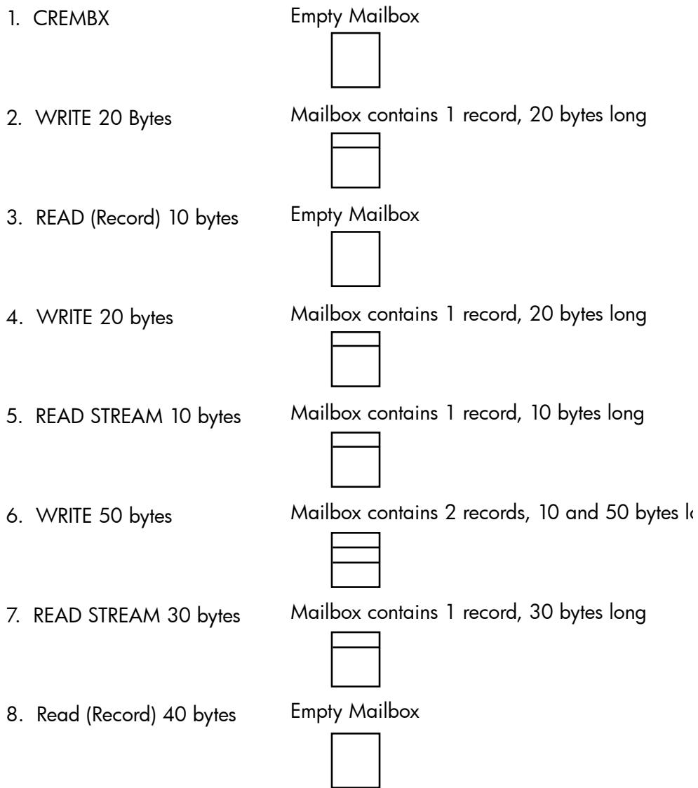
Figure 4-2 $QIO READ STREAM Operation
