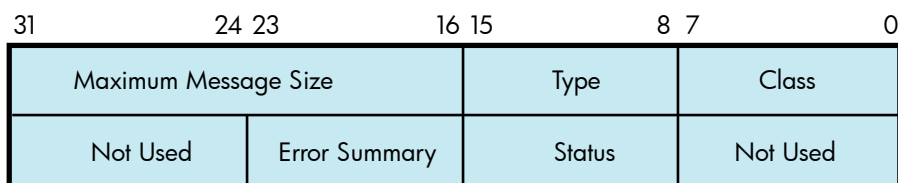
Figure 9-17 Sense Mode P1 Characteristics Buffer
