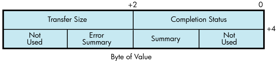
Figure 9-21 IOSB Contents
