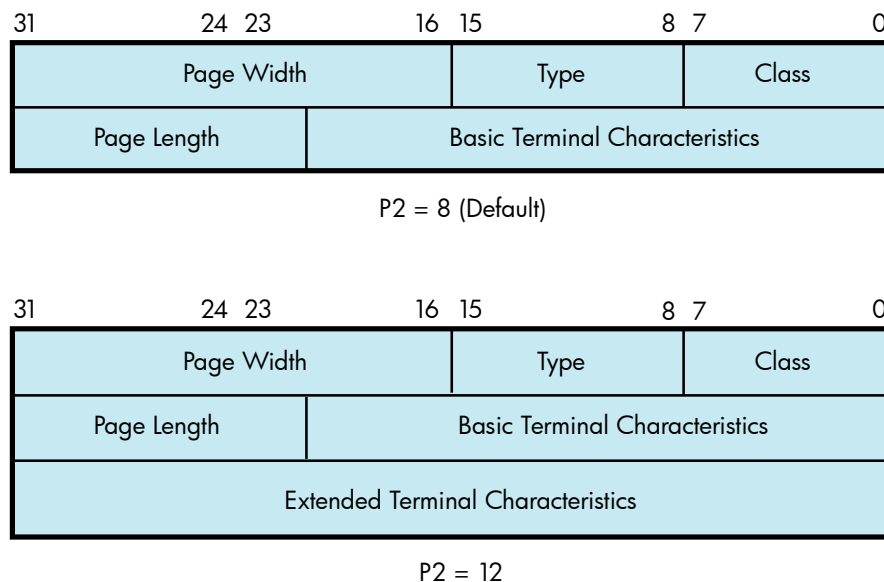
Figure 5-7 Set Mode and Set Characteristics Buffers
