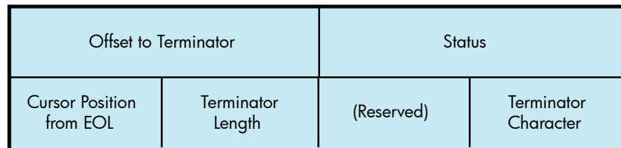
IOSB Contents: Itemlist Read Function
