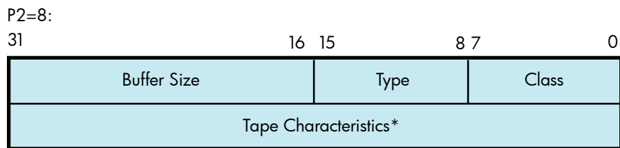
Figure 3-3 Sense Mode P1 Buffer
