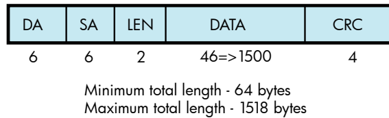
Figure 9-3 Ethernet Frame with IEEE 802.3 Header
