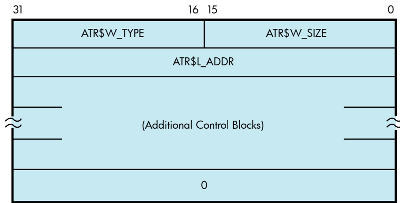
Figure 1-4 Attribute Control Block Format
