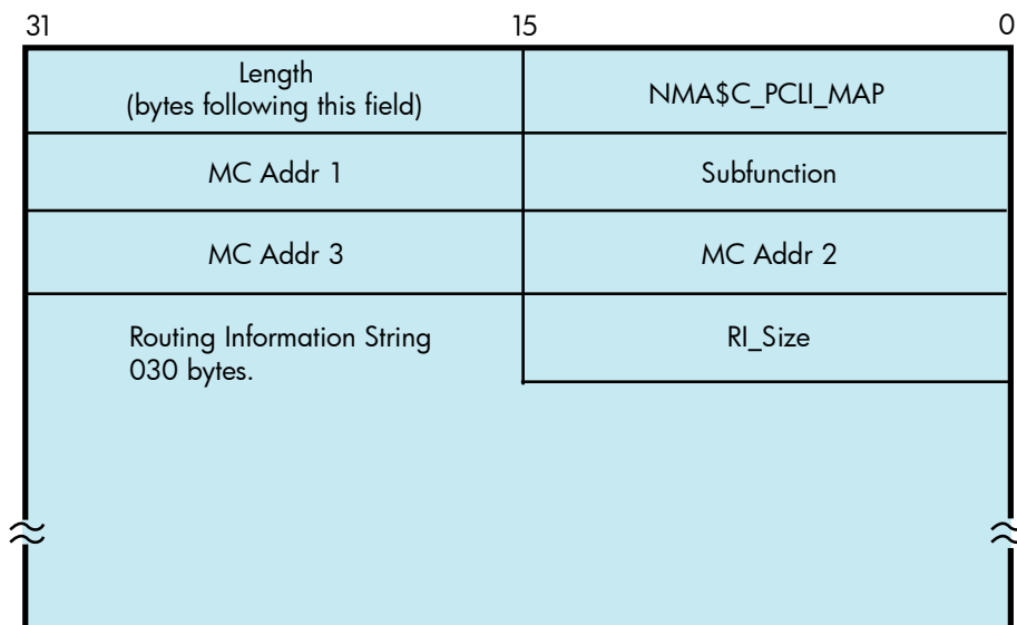
Figure 9-16 Format of the IO$M_ROUTE P2 Buffer
