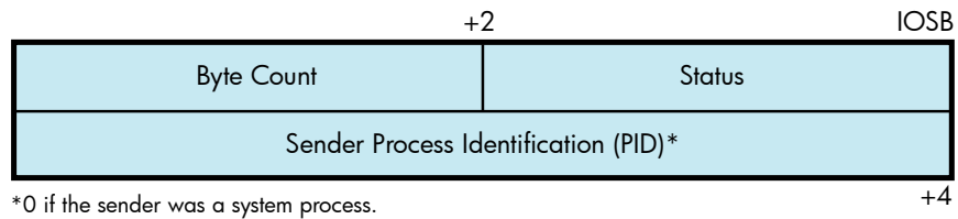
Figure 4-9 IOSB Contents— Write Function
