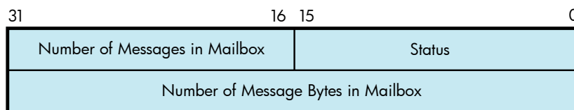
Figure 4-11 IOSB Contents — Get Mailbox Information Function
