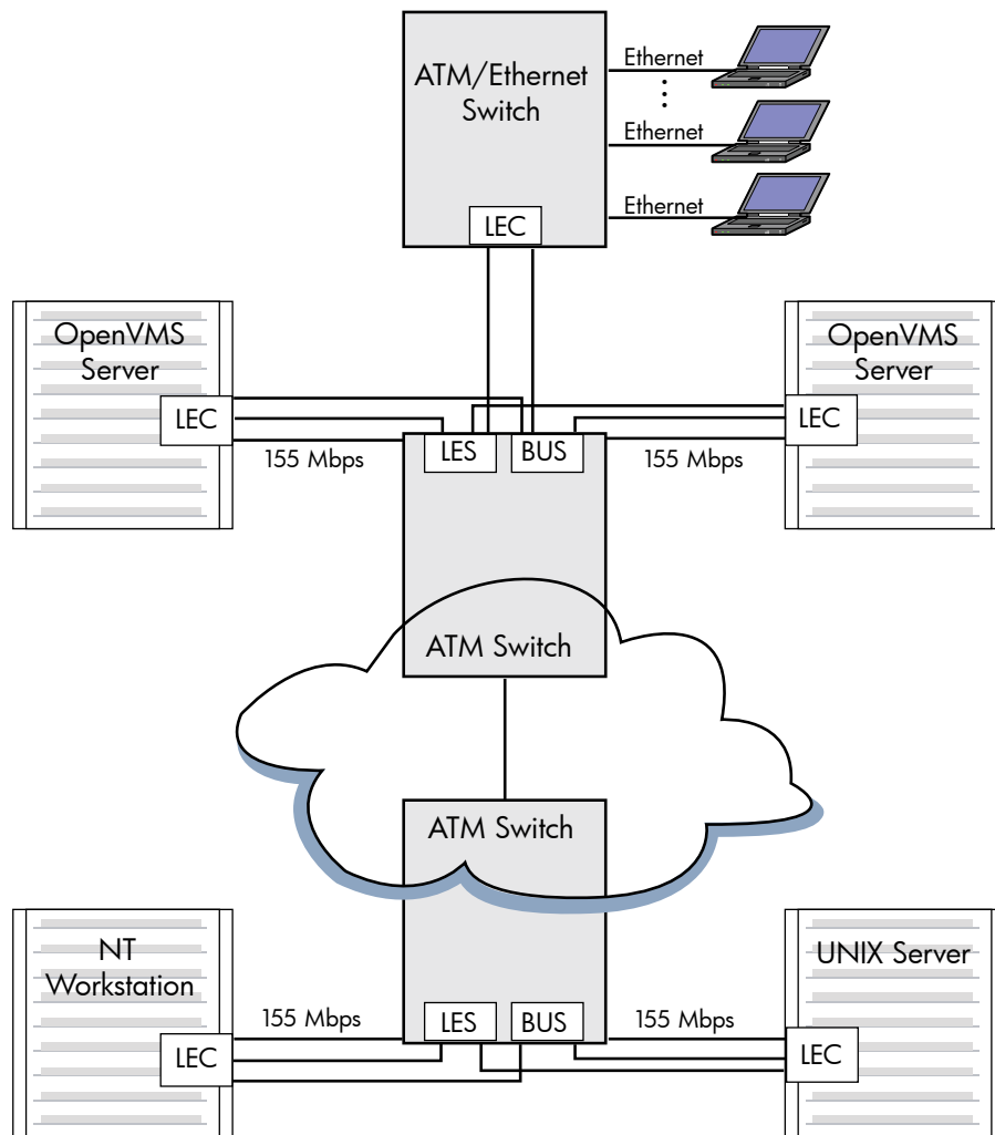
Figure 9-10 Emulated LAN Topology
