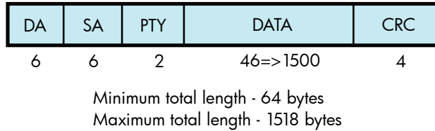
Figure 9-2 Ethernet Frame with Ethernet Header
