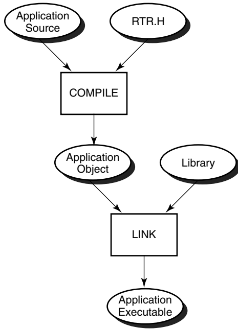
Figure 4-1 Compile Sequence
