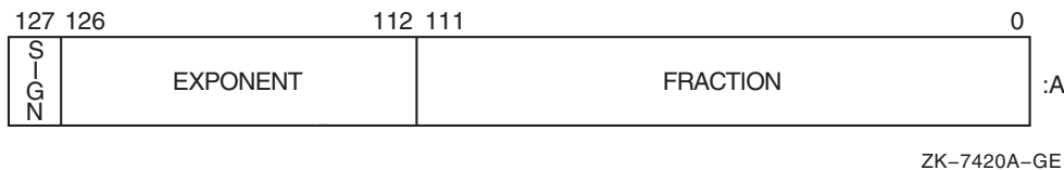
Figure 8–11 X_float REAL (KIND=16) Floating-Point Data Representation
