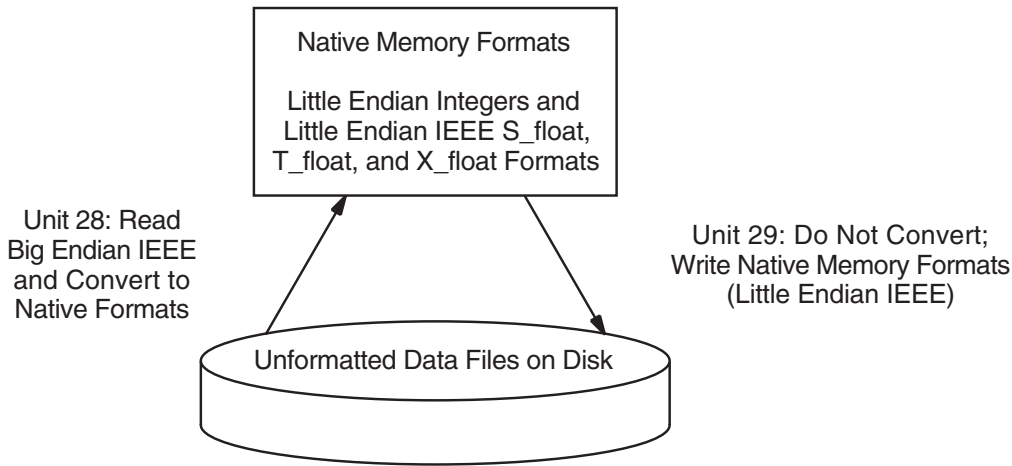
Figure 9–2 Sample Unformatted File Conversion
