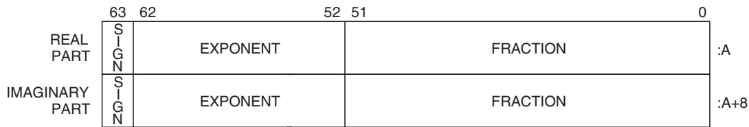
Figure 8–14 IEEE T_float COMPLEX (KIND=8) or COMPLEX*16 Representation
