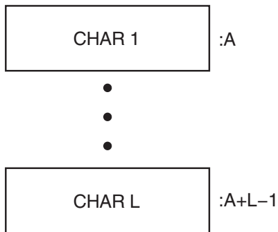
Figure 8–18 CHARACTER Data Representation
