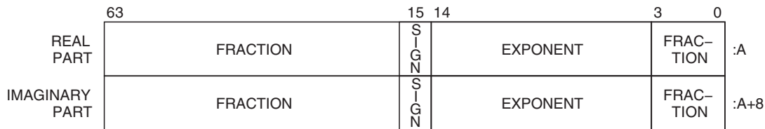
Figure 8–15 VAX G_float COMPLEX (KIND=8) or COMPLEX*16 Representation
