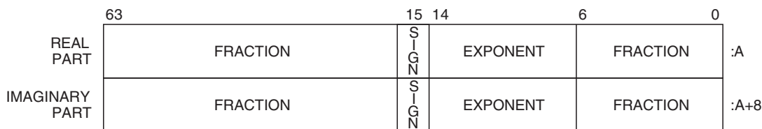
Figure 8–16 VAX D_float COMPLEX (KIND=8) or COMPLEX*16 Representation
