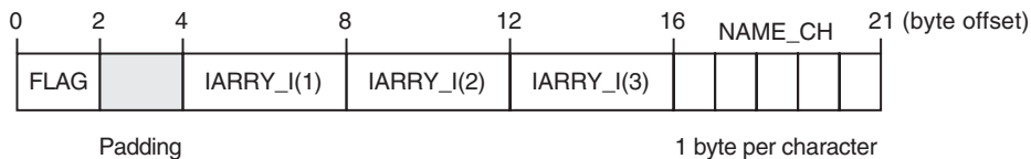
Figure 5-2 Common Block with Naturally Aligned Data
