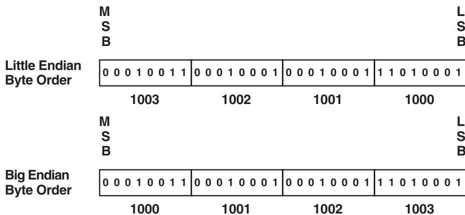
Figure 9–1 Little and Big Endian Storage of an INTEGER Value
