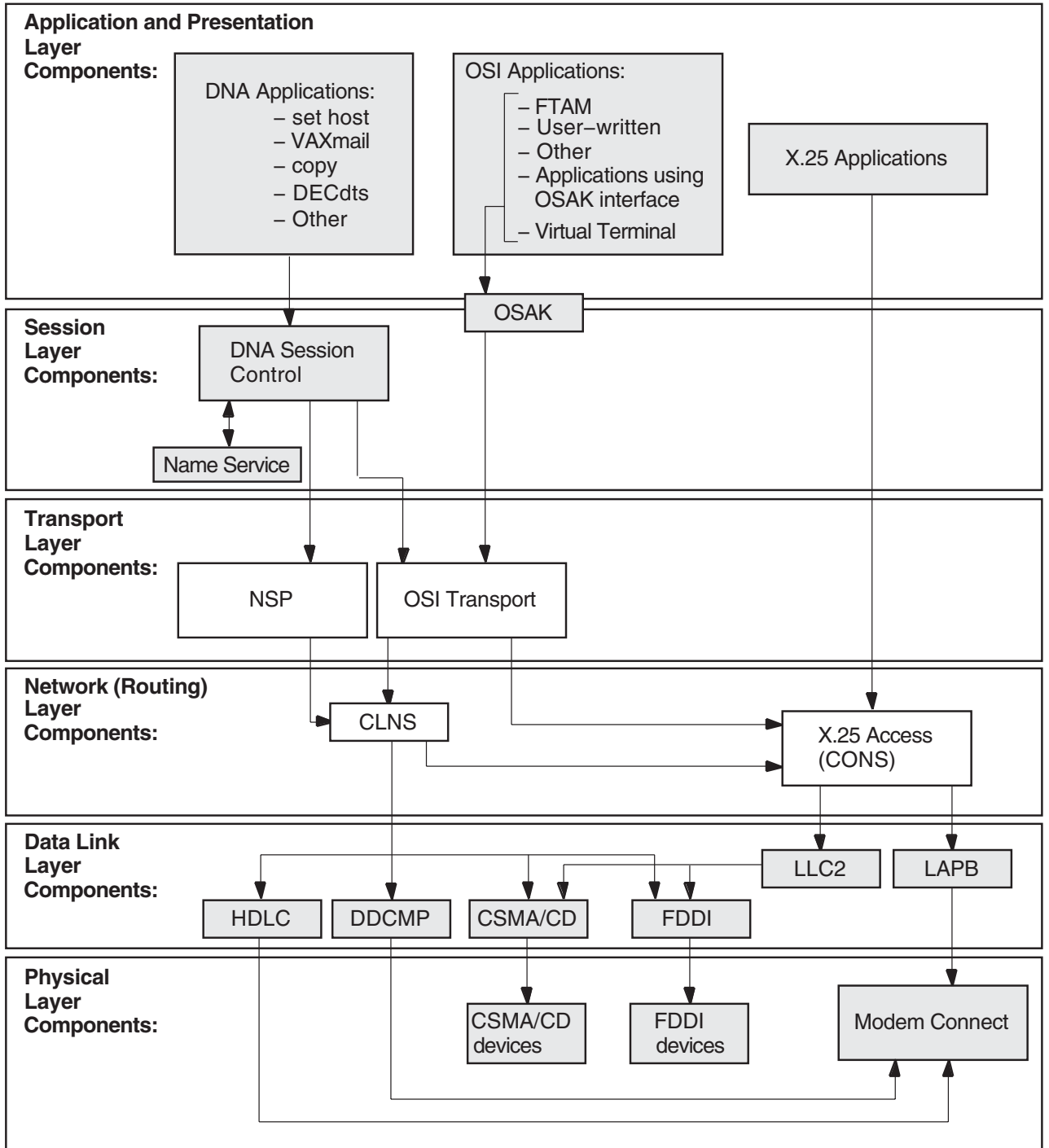
Figure 7-1 Underlying Components (OpenVMS)
