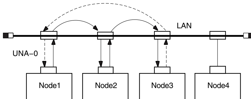
Figure 3-5 Circuit-Level Loopback Test with Transmit Assistance
