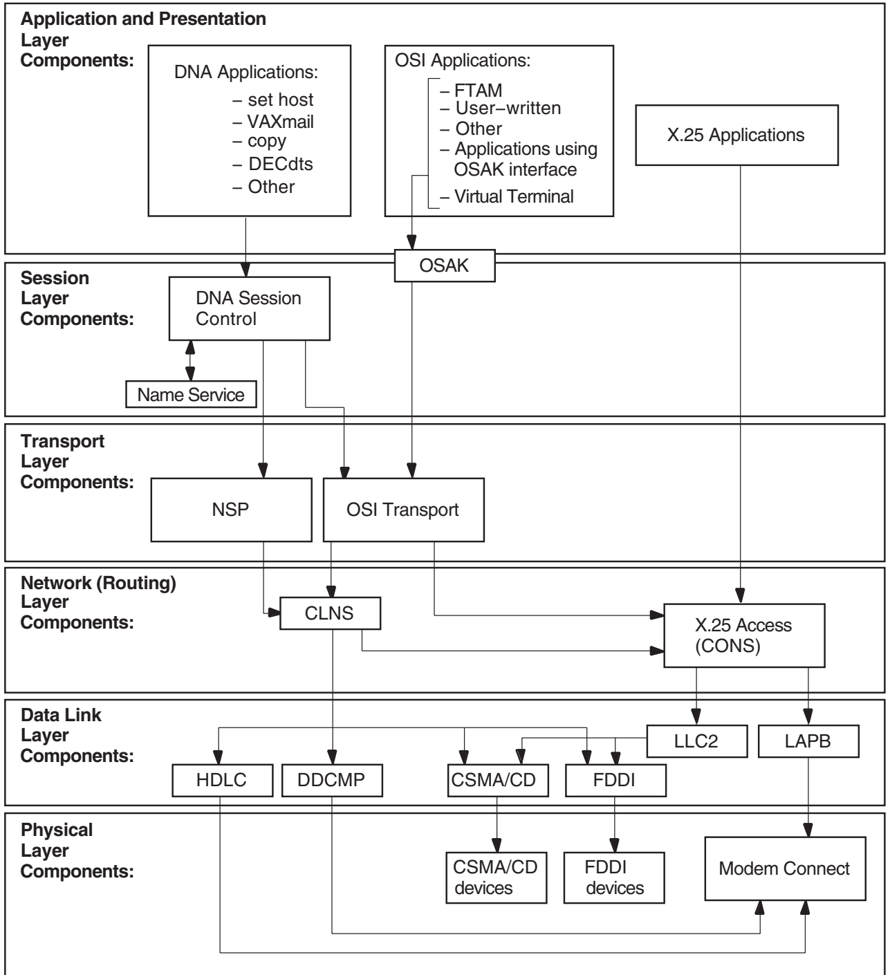
Figure 1-2 Component Relationships (OpenVMS)
