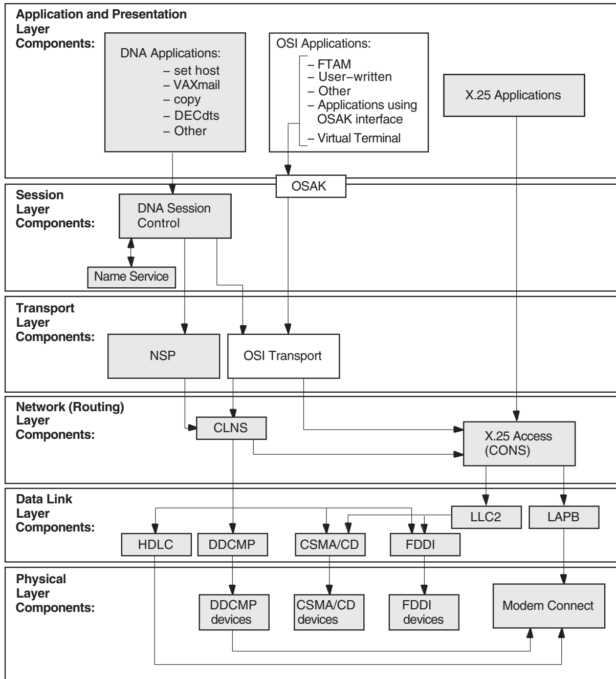
Figure 5-1 Underlying DECnet-Plus Components (OpenVMS)
