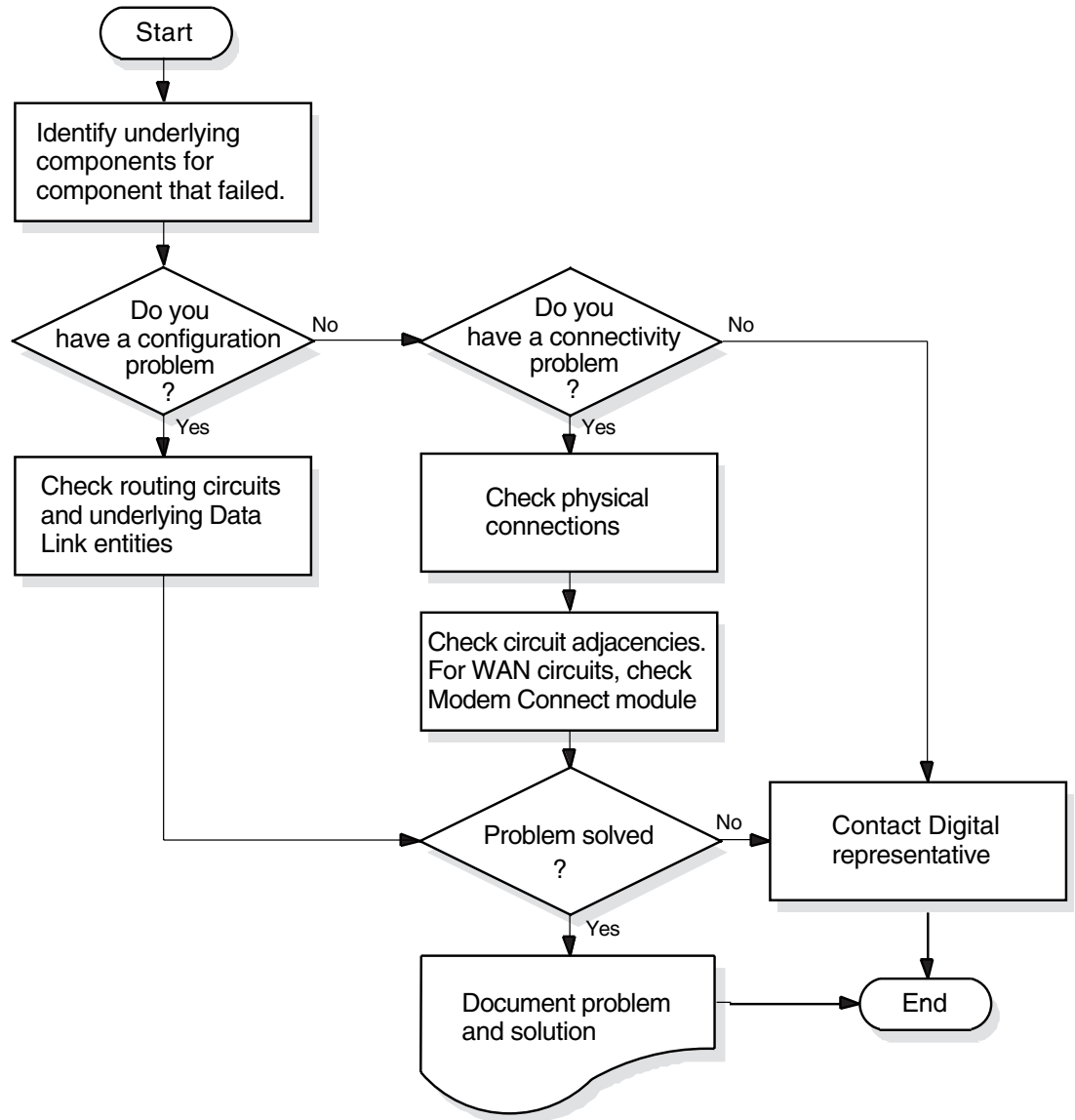
Figure 8–3 Fault-Isolation Methodology (Circuit Connectivity)
