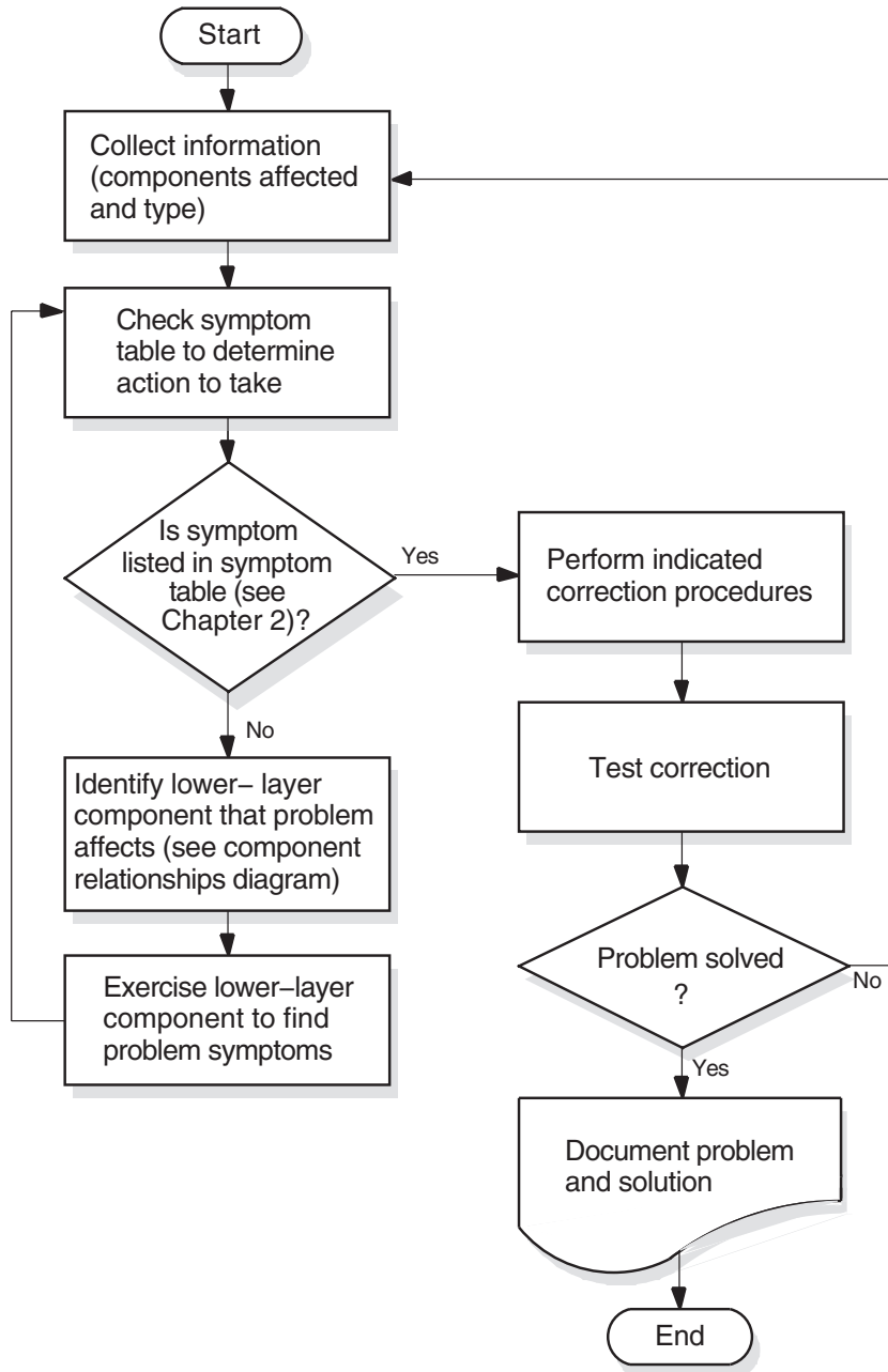
Figure 1-4 Fault-Isolation Methodology (General)
