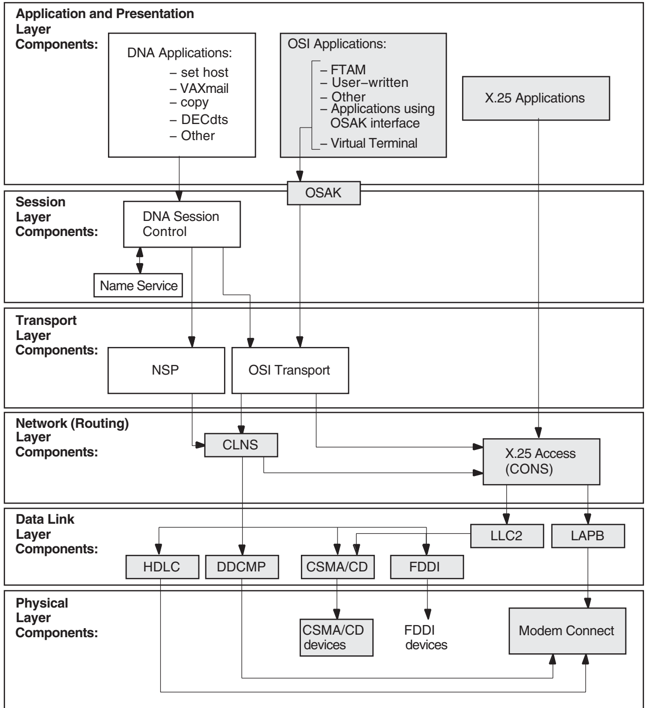
Figure 6-1 Underlying Components for Session Control (OpenVMS)
