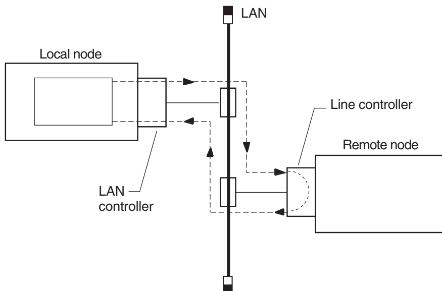
Figure 3-3 Circuit-Level Loopback Test
