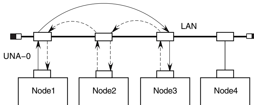
Figure 3-6 Circuit-Level Loopback Test with Receive Assistance
