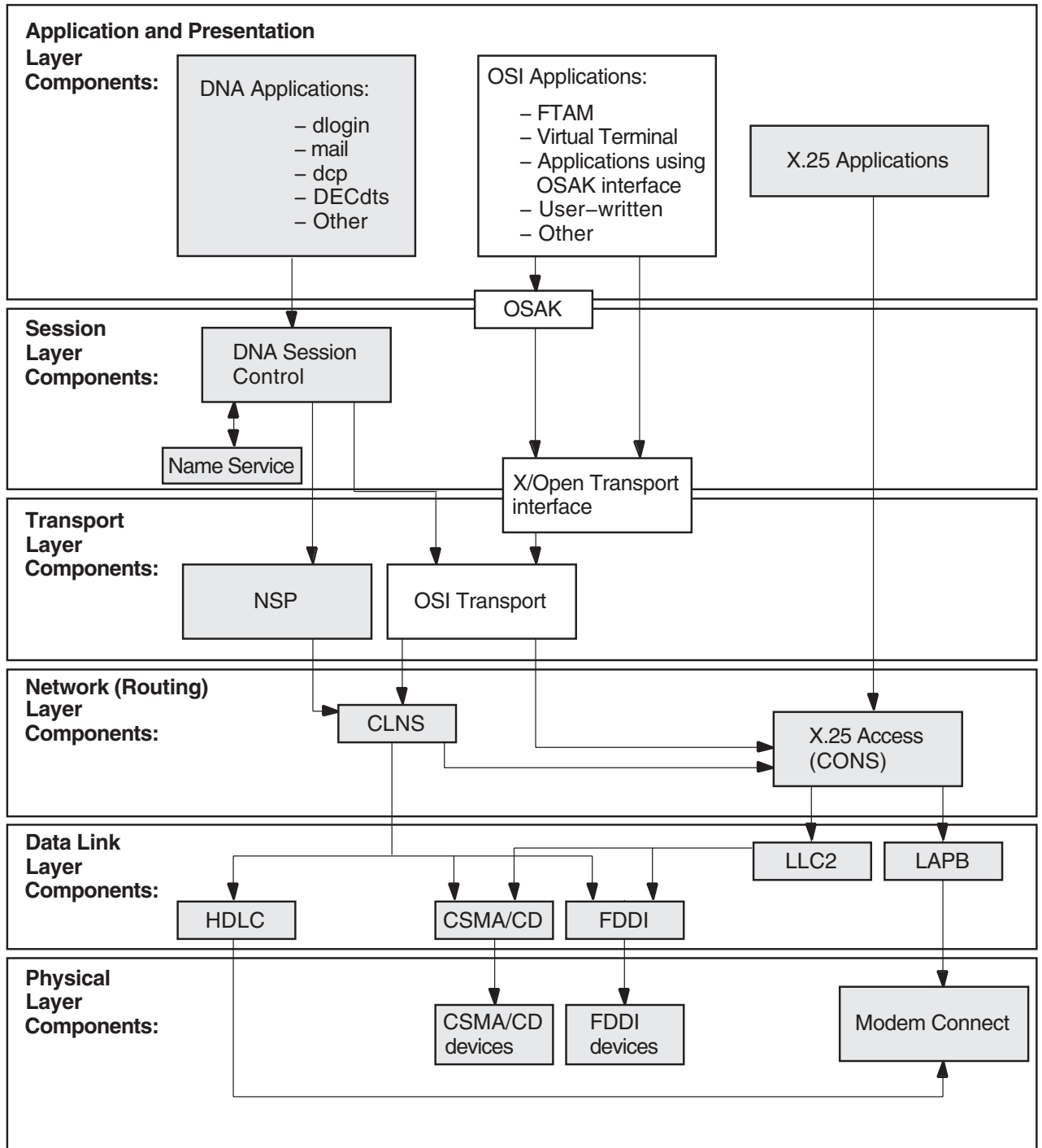
Figure 5-2 Underlying DECnet/OSI Components (Digital UNIX)
