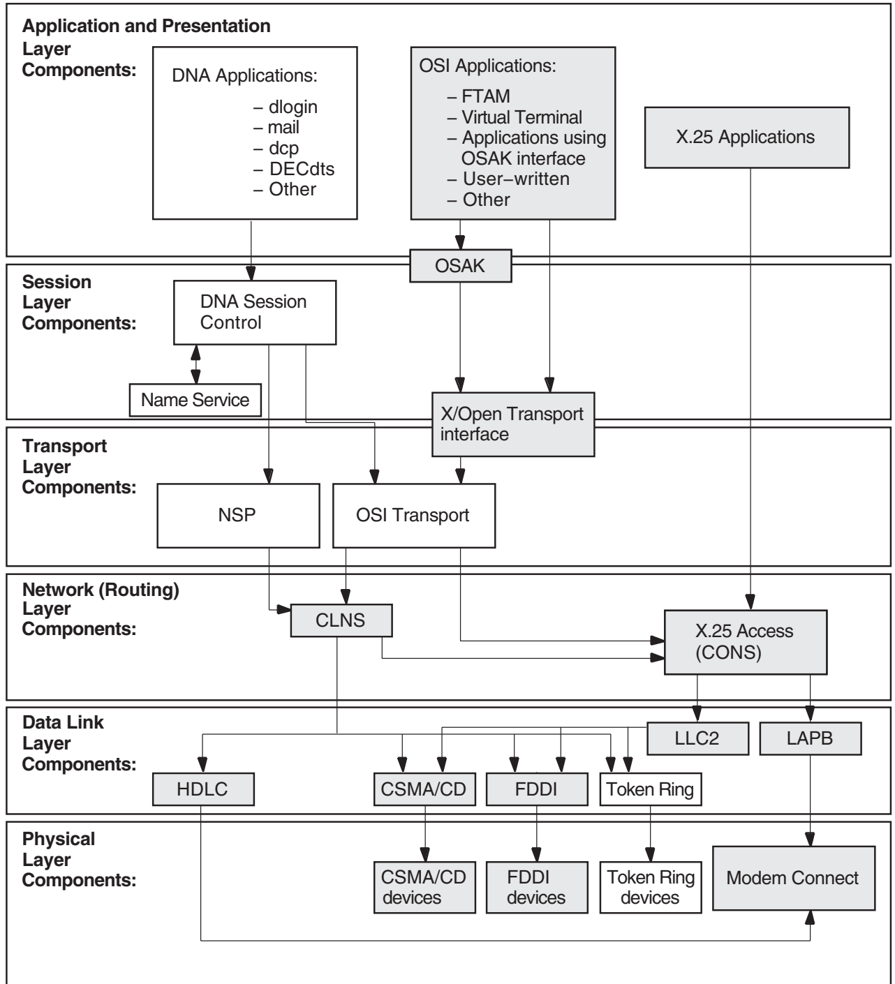
Figure 6-2 Underlying Components for Session Control (Digital UNIX)
