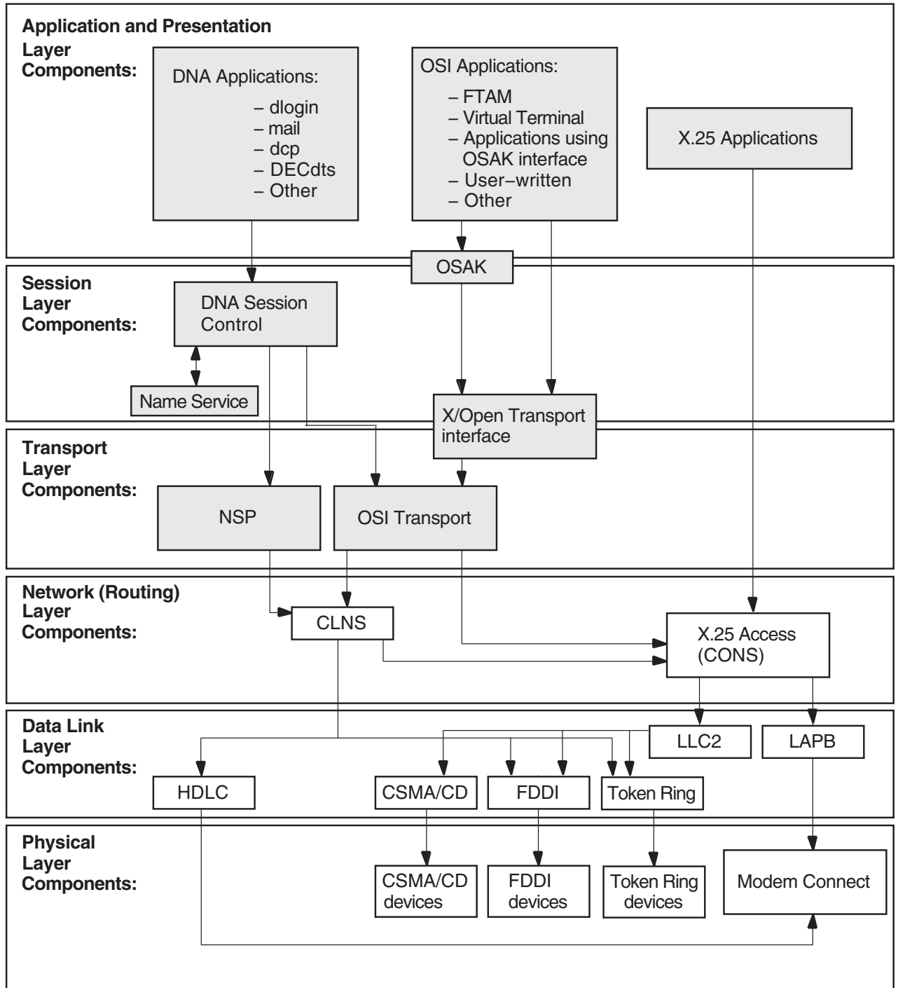
Figure 8-2 Underlying Entities (Digital UNIX)
