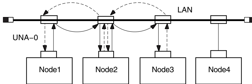
Figure 3-4 Circuit-Level Loopback Test with Full Assistance
