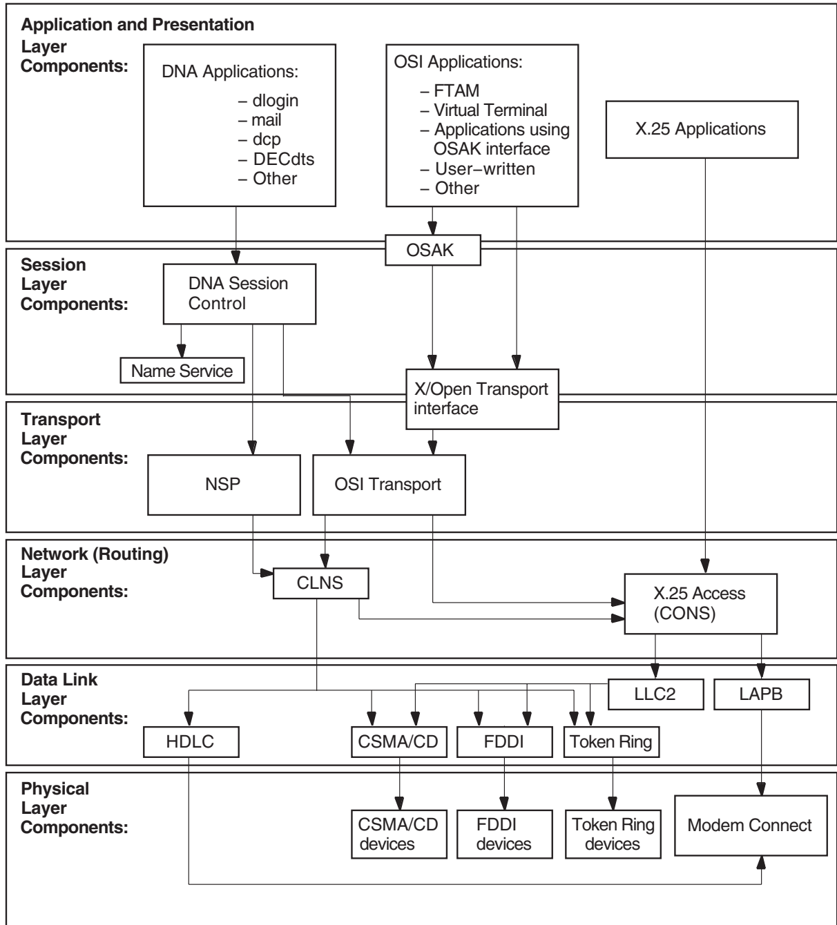
Figure 1-3 Component Relationships (Digital UNIX)
