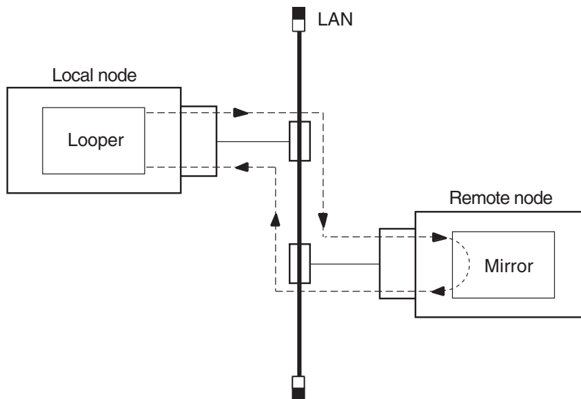
Figure 3–2 Local-to-Remote Loopback Test
