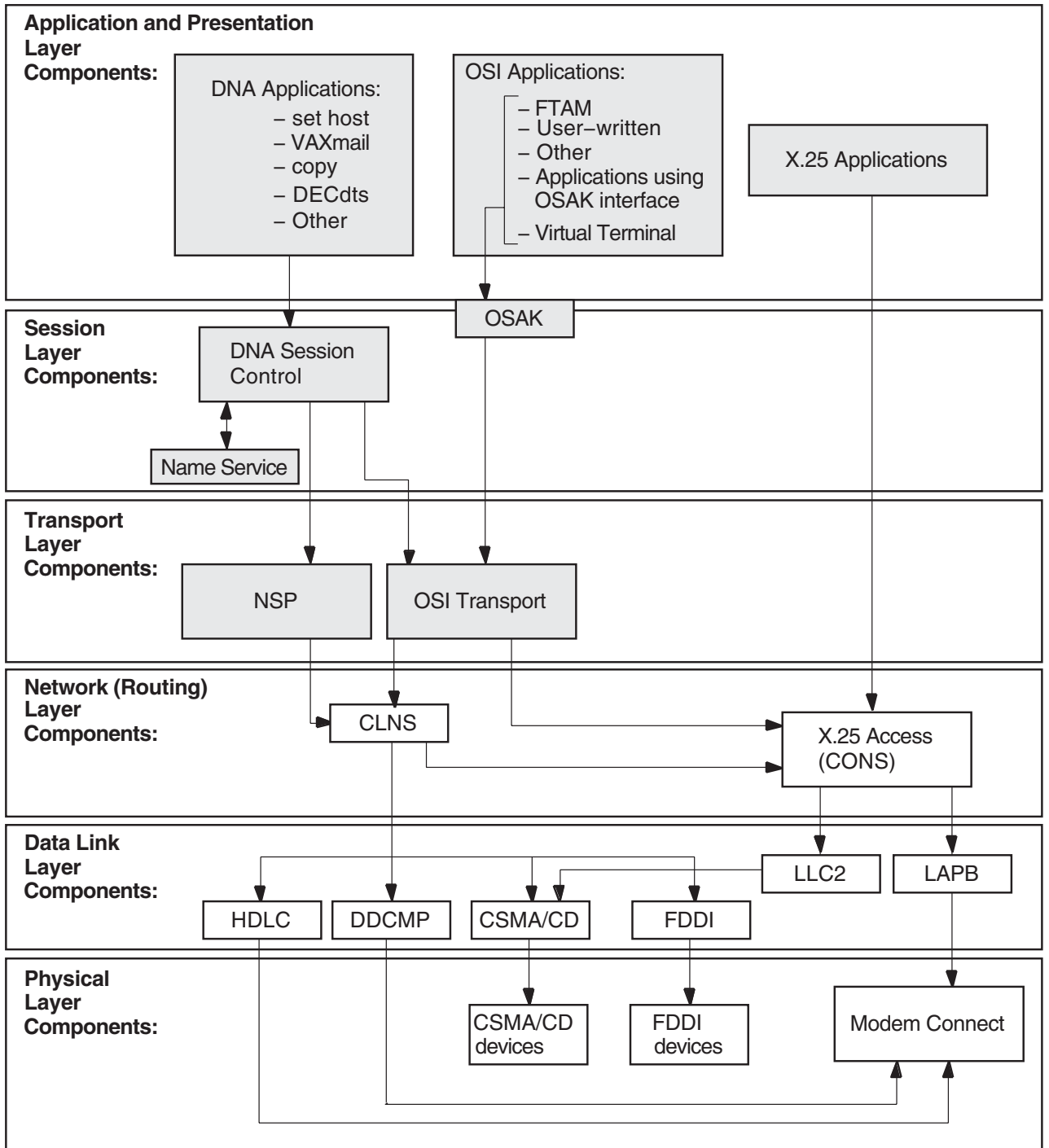
Figure 8-1 Underlying Entities (OpenVMS)
