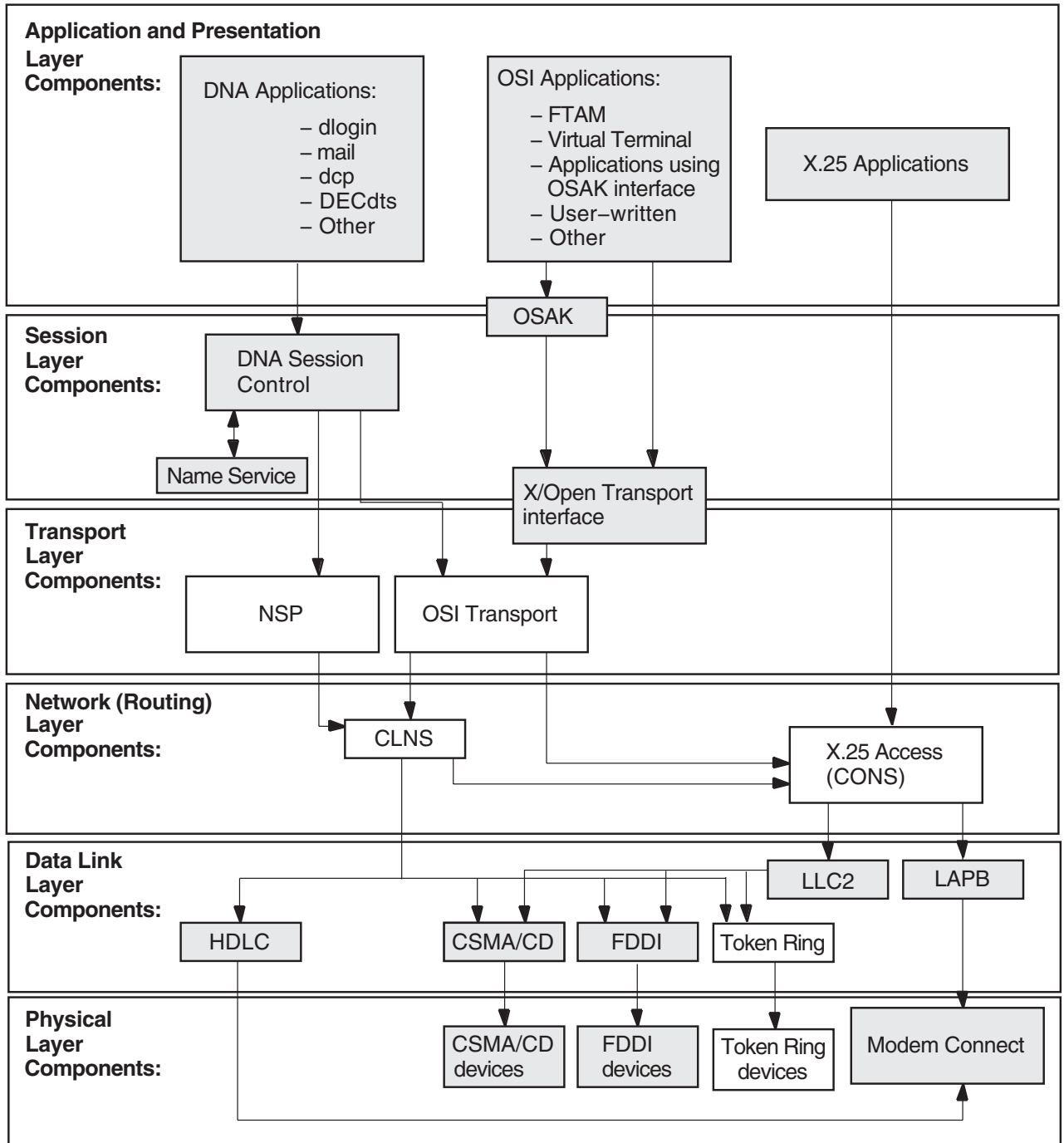
Figure 7-2 Underlying Components (Digital UNIX)
