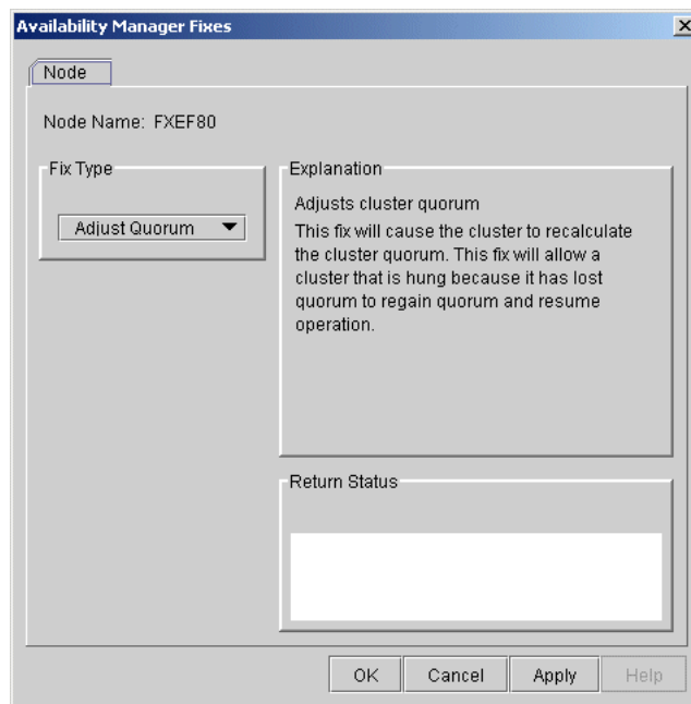
Figure 6–1 Adjust Quorum
