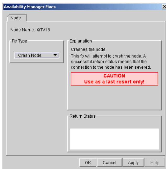
Figure 6–2 Crash Node
