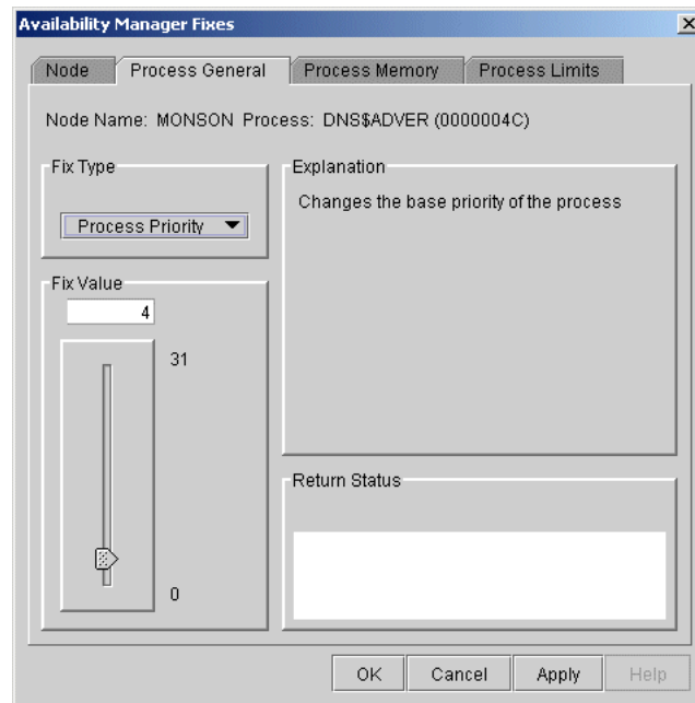
Figure 6–8 Process Priority
