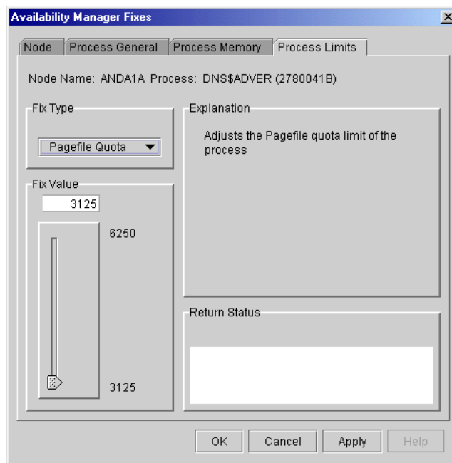
Figure 6–19 Pagefile Quota
