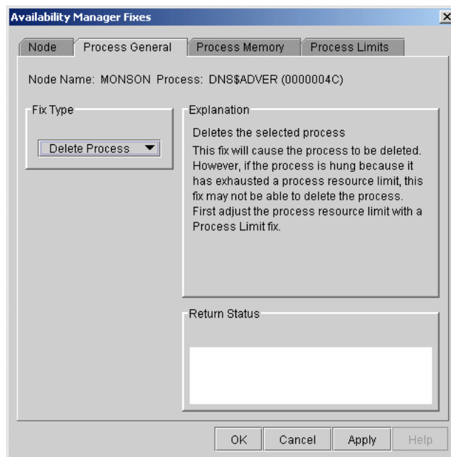
Figure 6–4 Delete Process
