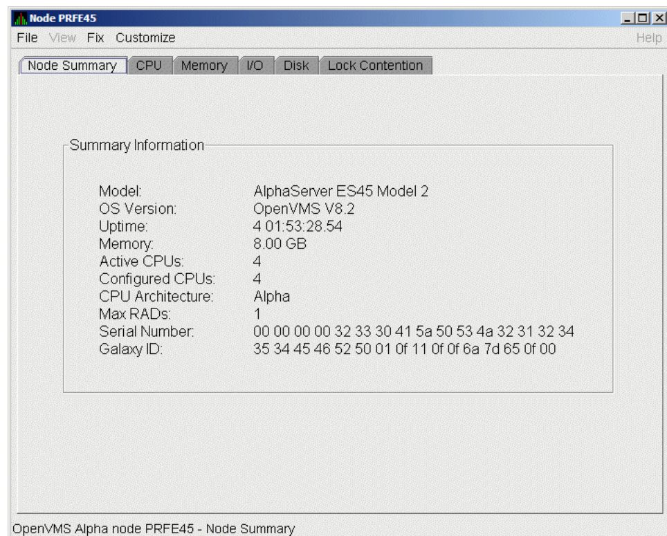
Figure 3–4 Node Summary
