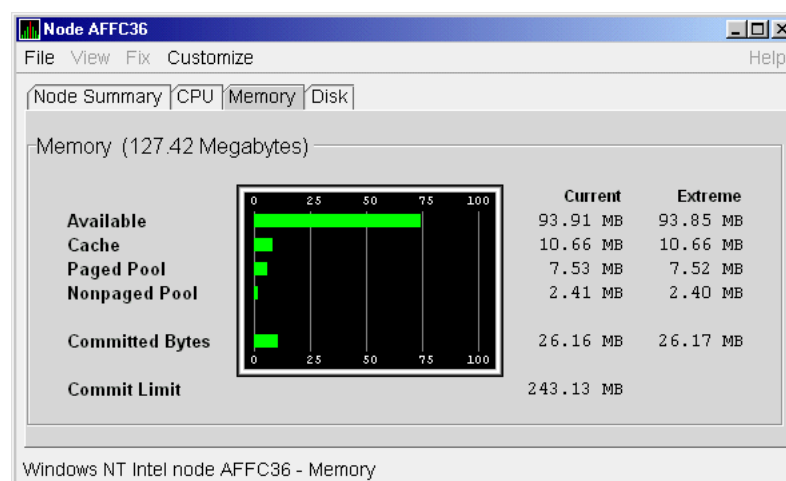
Figure 3–9 Windows Memory
