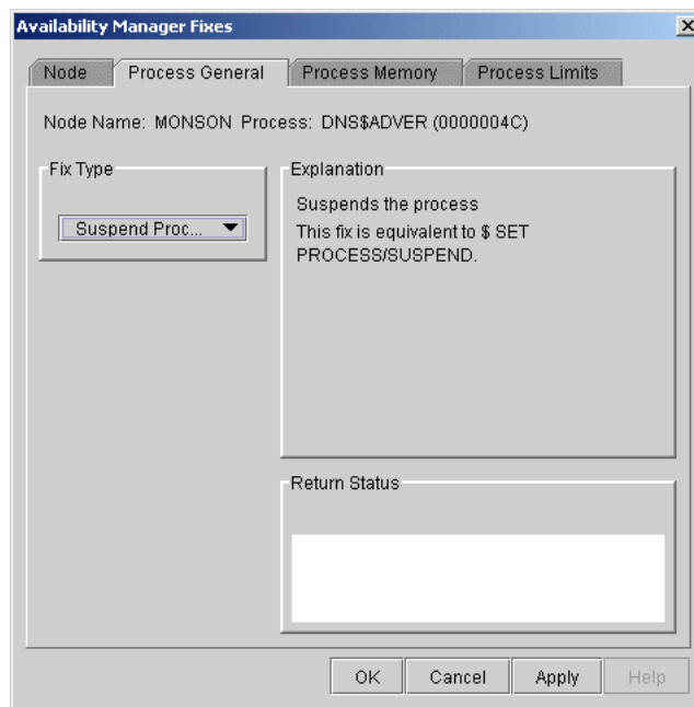
Figure 6–6 Suspend Process
