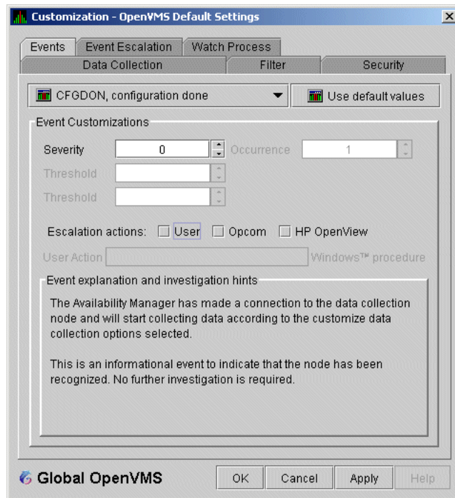
Figure 7–19 Event Customizations
