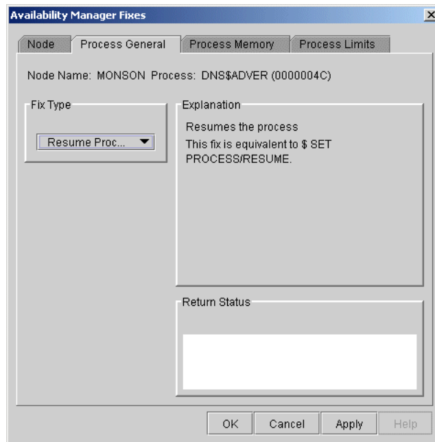
Figure 6–7 Resume Process
