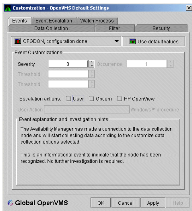
Figure 7–18 Event Customizations
