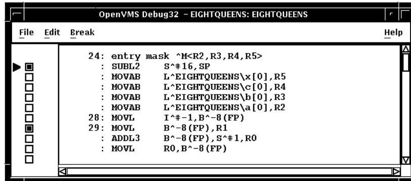
Figure 10–21 Instruction View
