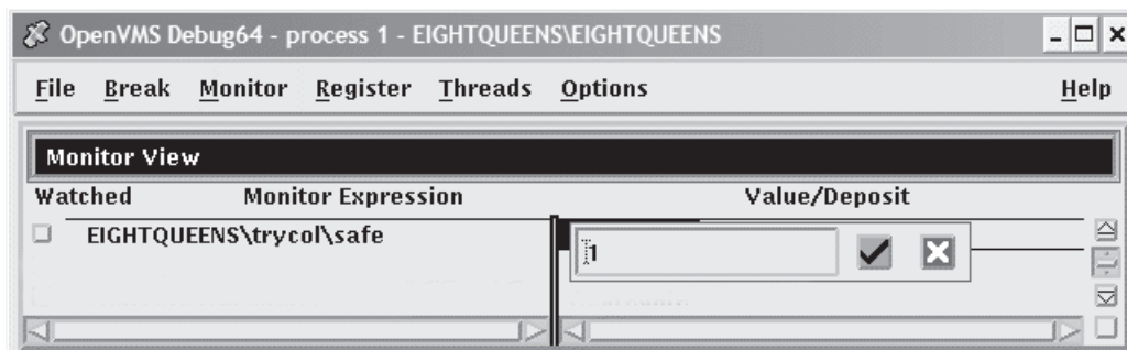
Figure 10–17 Changing the Value of a Monitored Scalar Variable
