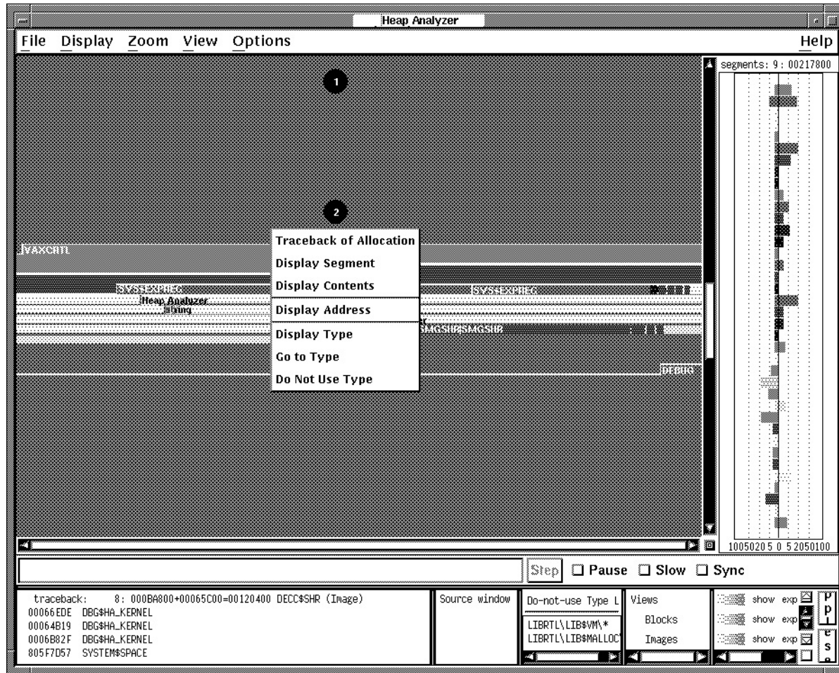
Figure 12–6 Heap Analyzer Memory Map Context-Sensitive Pop-Up Menu
