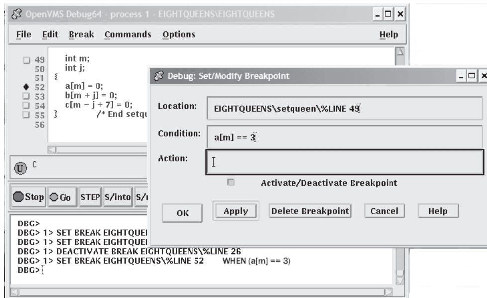
Figure 10–6 Setting a Conditional Breakpoint
