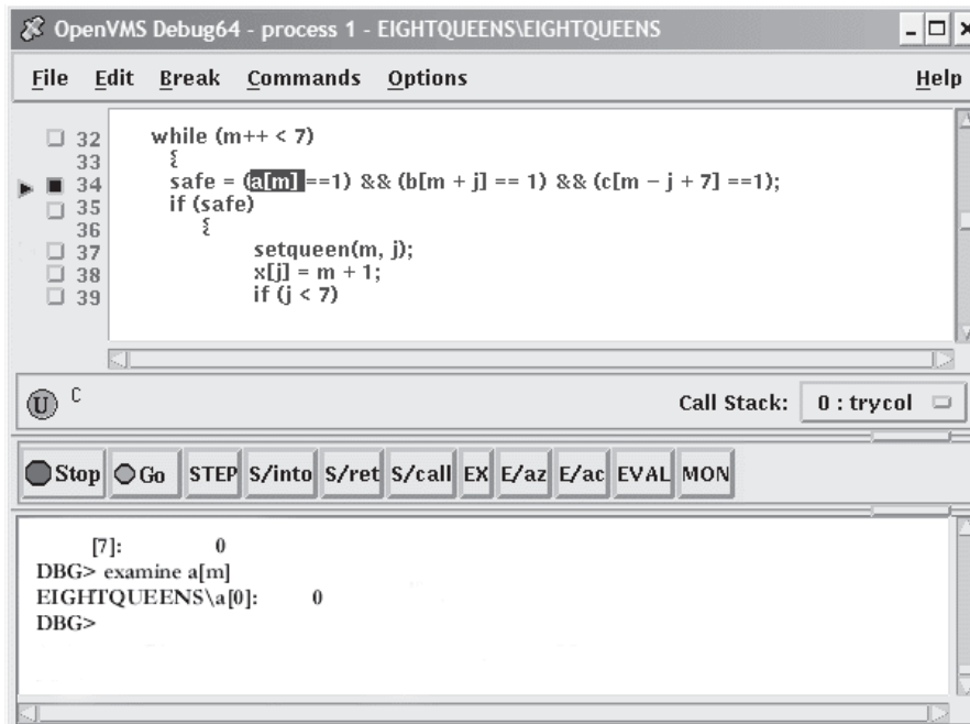
Figure 10–11 Typecasting the Value of a Variable
