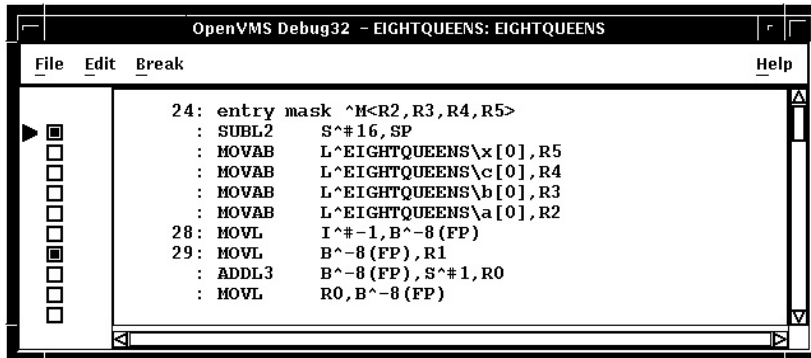
Figure 8–7 Tasking View
