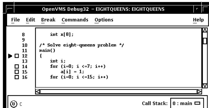
Figure 10–1 Source Display
