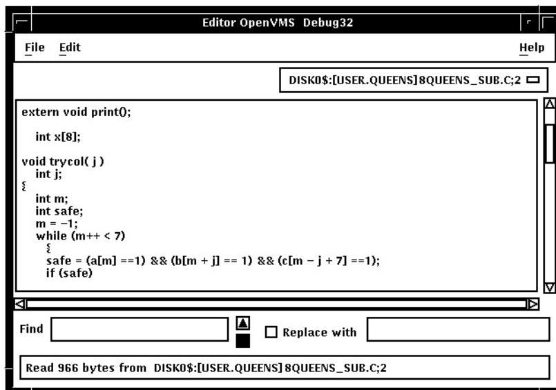
Figure 10–3 Editor Window
