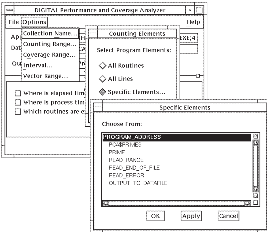
Figure 2-5 Specific Elements List Box
