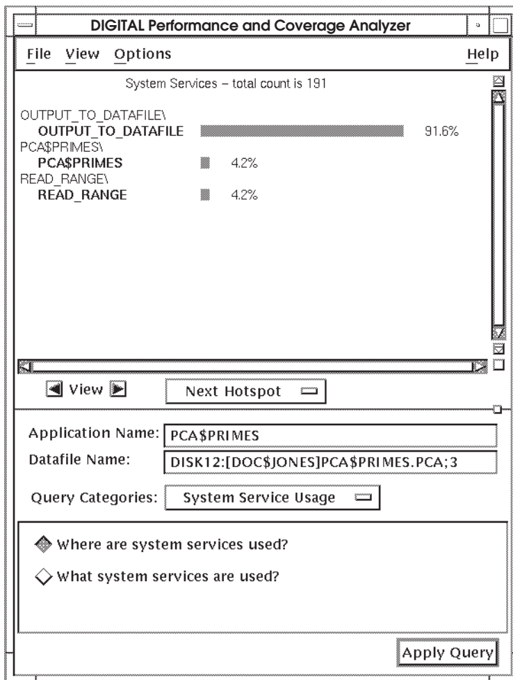
Figure 7–1 Histogram Showing Where System Services Are Used
