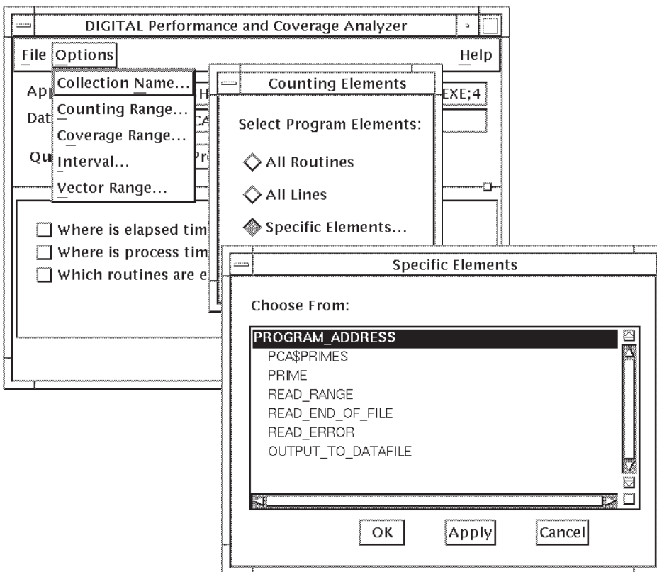
Figure 5-1 Selecting Execution Counts for a Specific Routine
