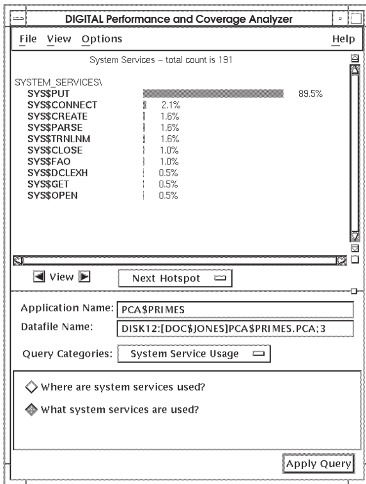
Figure 7–3 Histogram Showing What System Services Are Used
