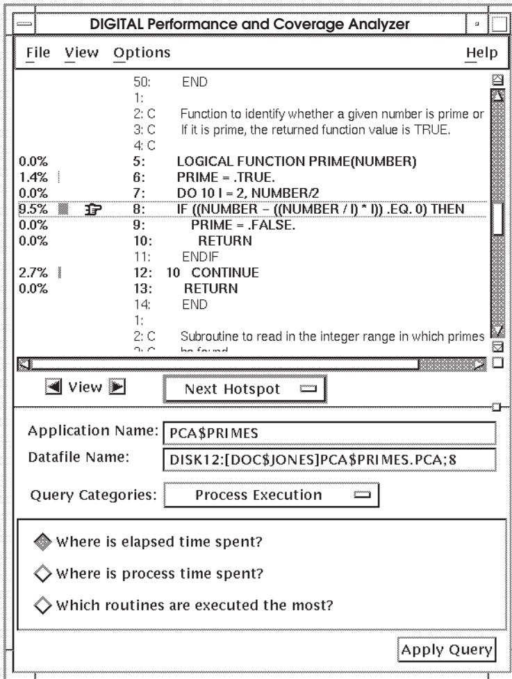
Figure 3–5 Sample Annotated Source Listing
