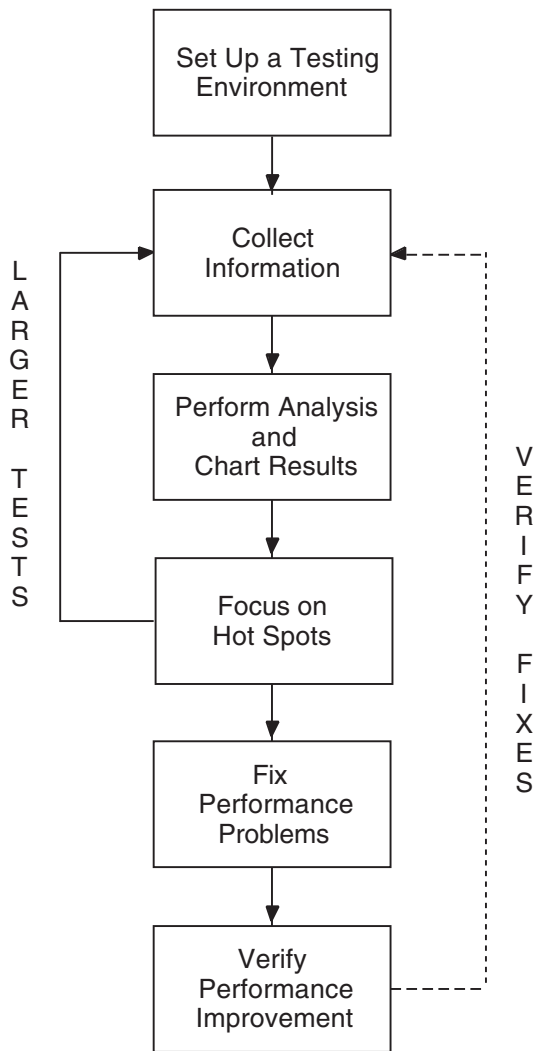
Figure 1-5 PCA Usage Methodology
