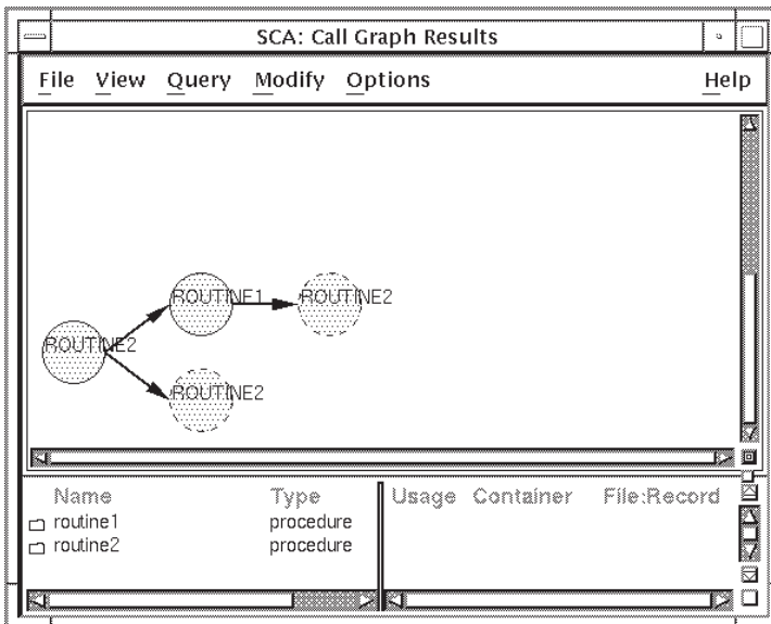
Figure 4–12 Recursive Calls
