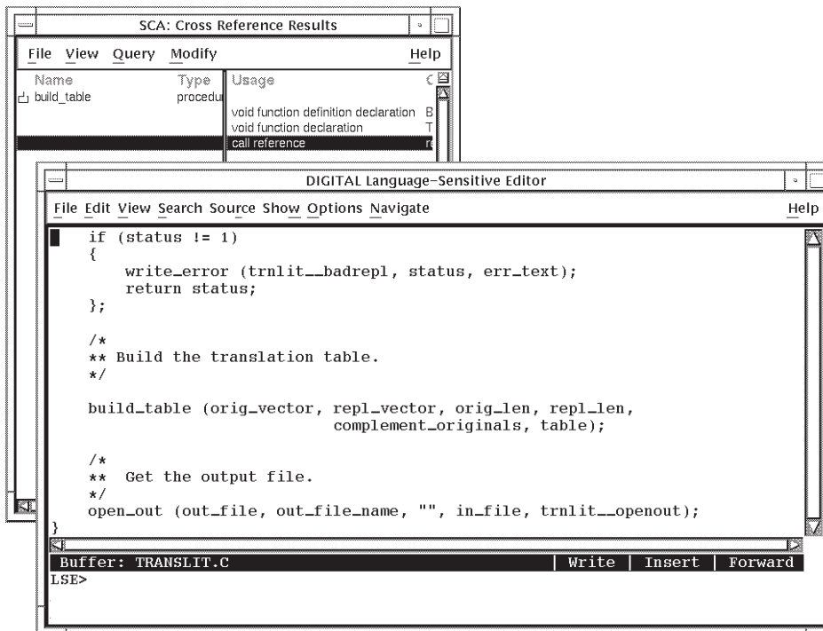
Figure 4-4 Go-To-Source Feature
