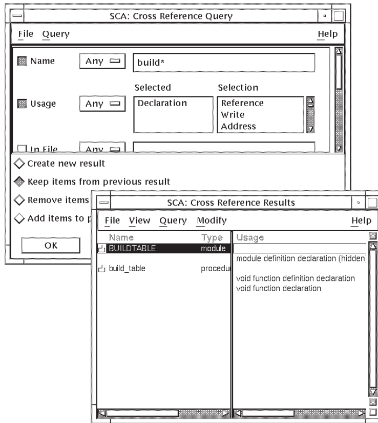
Figure 4–19 Keeping Items from the Results
