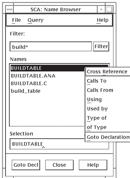
Figure 2–1 Name Browser Dialog Box
