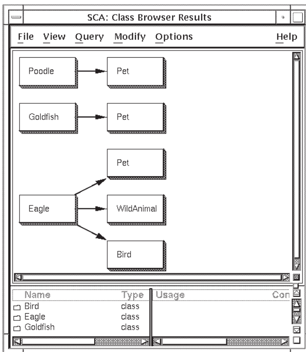
Figure 2–5 Extending to a Class Node
