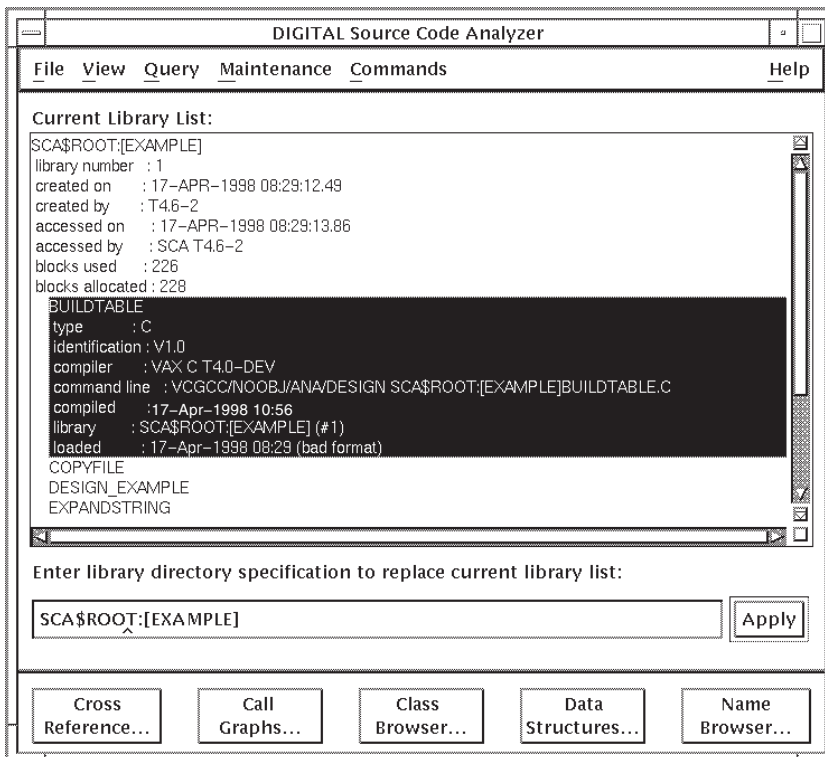
Figure 3-5 Displaying Attributes
