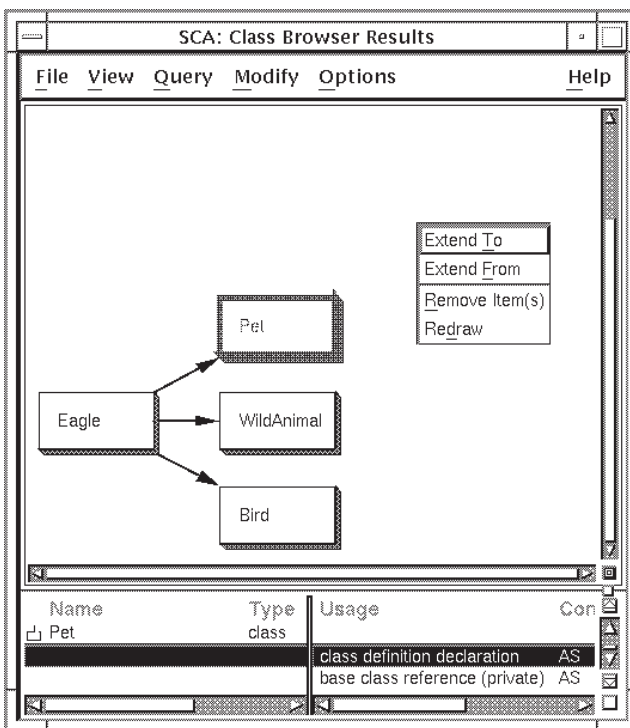
Figure 2–4 The Class Browser Results Window
