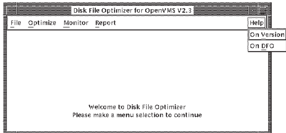
Figure 5–1 Initial Window
