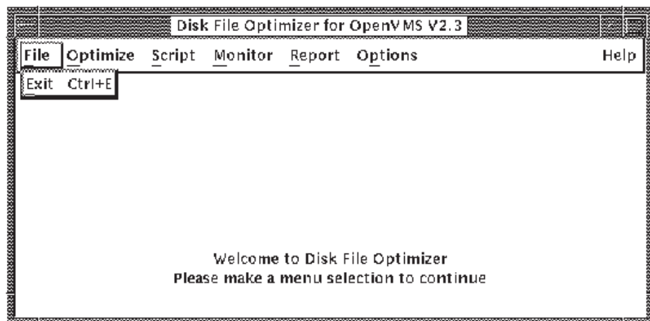
Figure 6–2 File Menu
