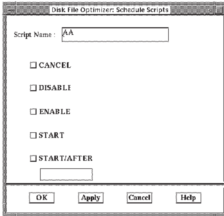
Figure 6-14 Schedule Script
