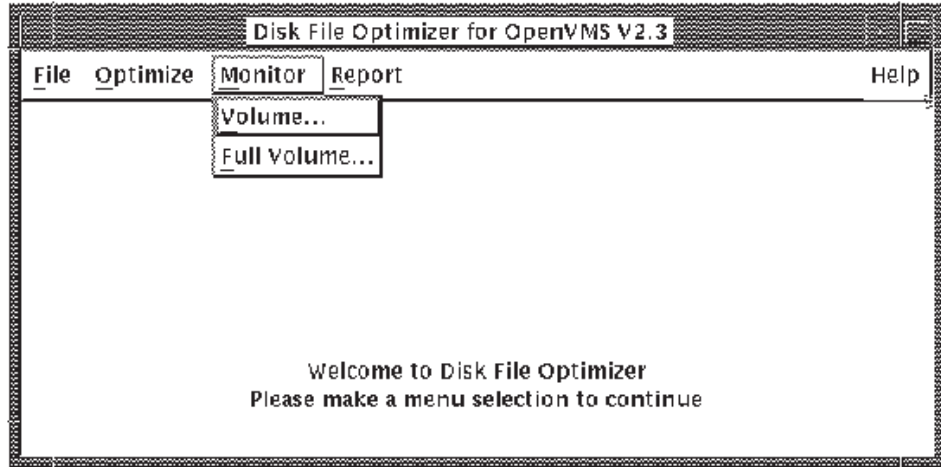
Figure 5–10 Monitor Menu
