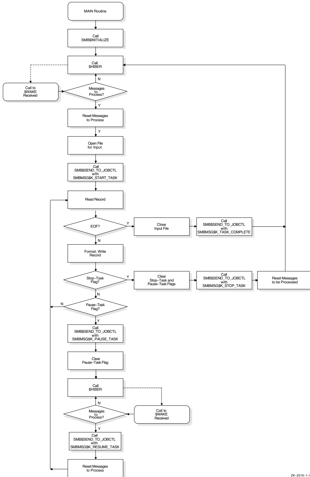
Figure 18–3 Flowchart for a Single-Threaded, Asynchronous Symbiont (MAIN Routine)
