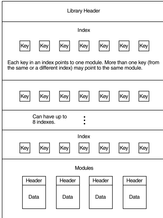
Figure 12–3 Structure of a User-Developed Library
