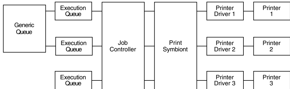
Figure 17–1 Multithreaded Symbiont
