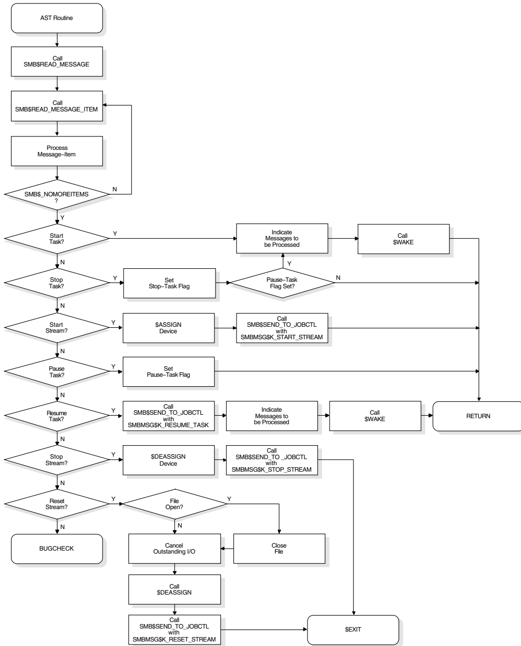
Figure 18–4 Flowchart for a Single-Threaded, Asynchronous Symbiont (AST Routine)
