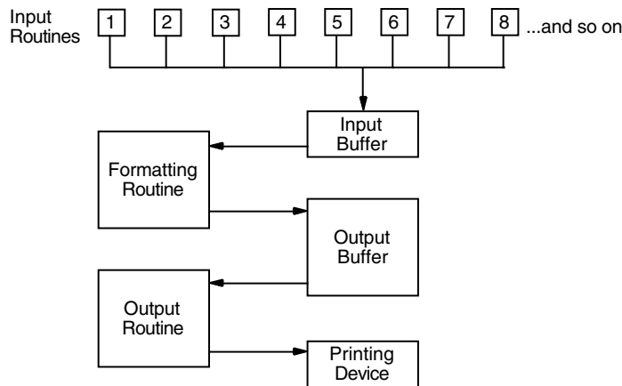
Figure 17–2 Symbiont Execution Sequence or Flow of Control
