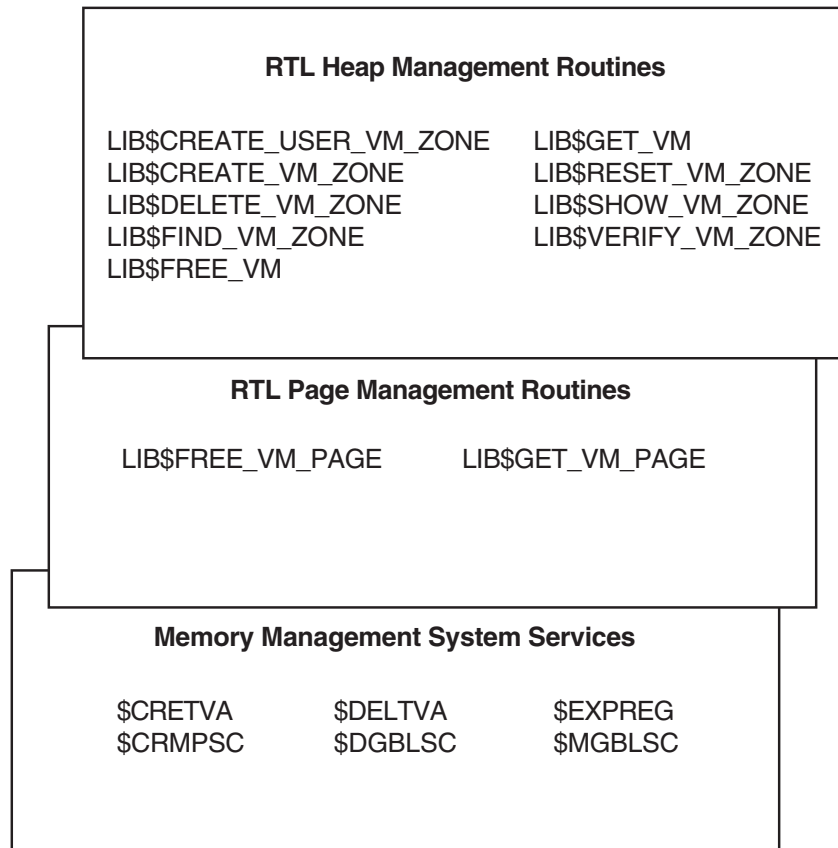
Figure 12–1 Hierarchy of Alpha Memory Management Routines
