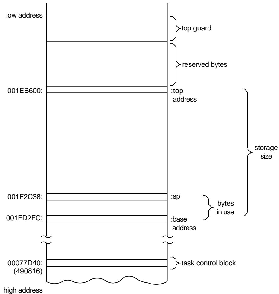
Figure 17–1 Diagram of a Task Stack
