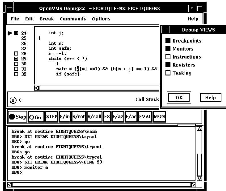
Figure 8–4 Debugger Main Window
