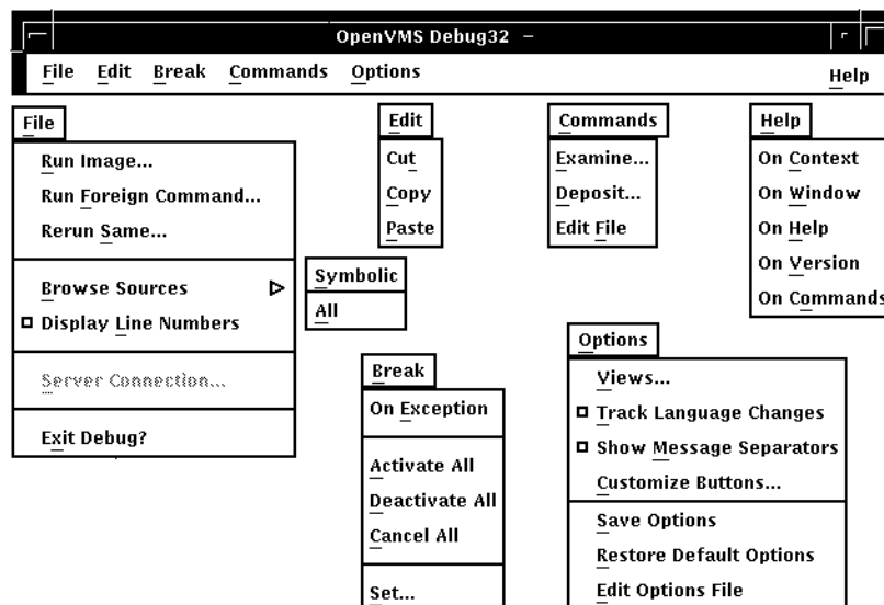
Figure 8–2 Menus on Main Window
