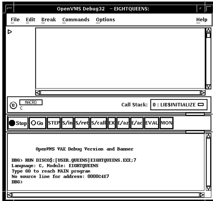
Figure 9-4 Source Display at Startup
