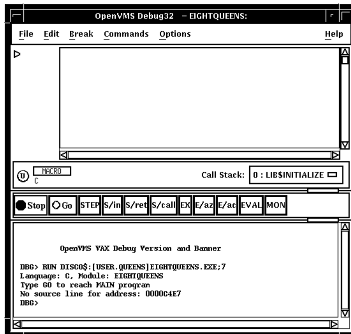
Figure 8–1 Default Window Configuration
