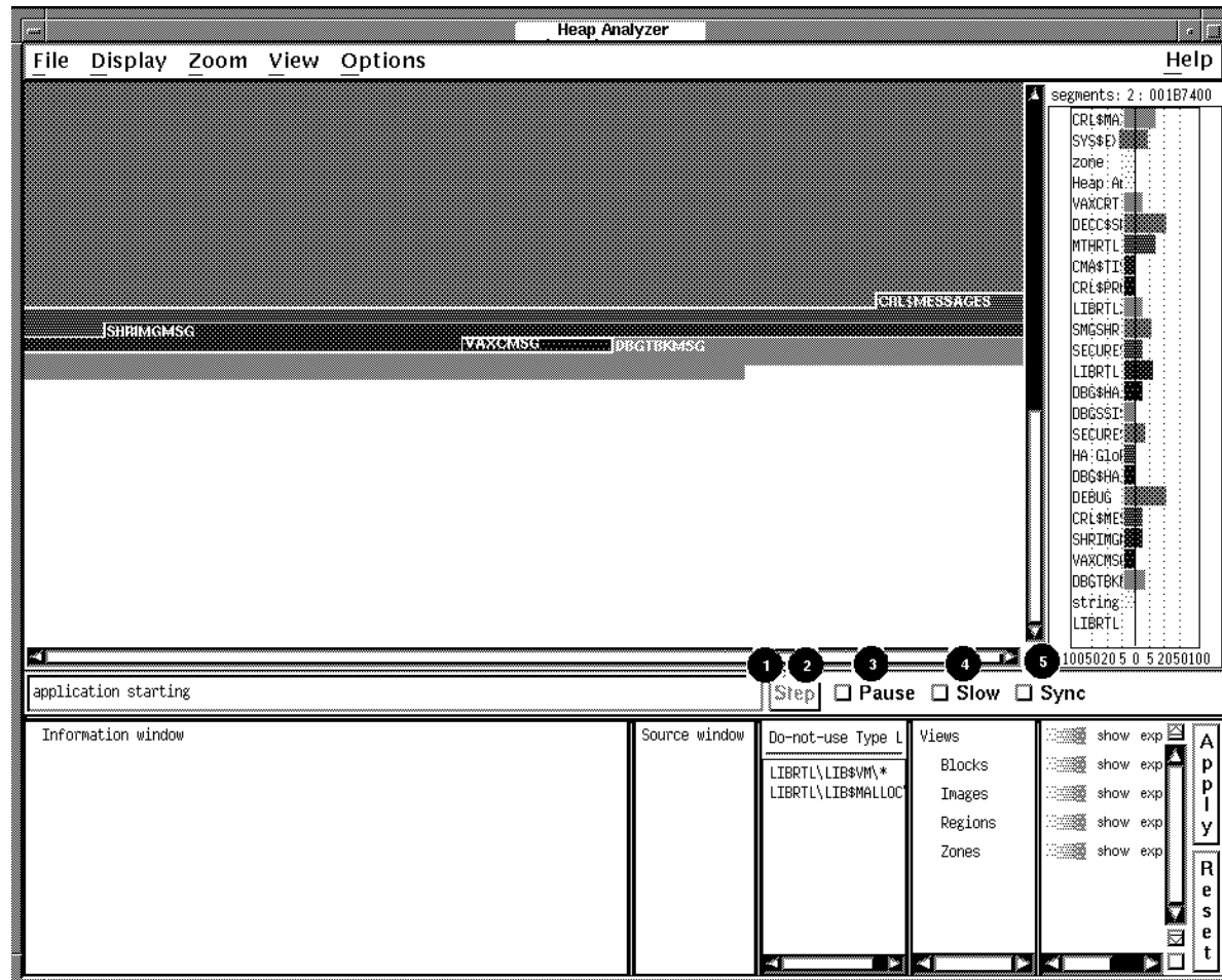
Figure 12–4 Heap Analyzer Control Panel
