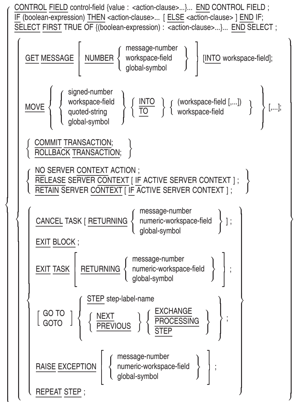
Figure 3–10 Action Syntax
