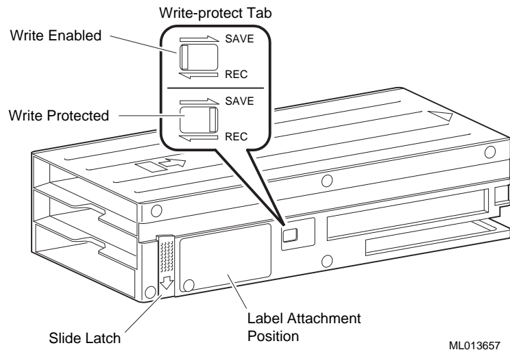
Figure 7-5 TLZ9L Cassette Magazine
