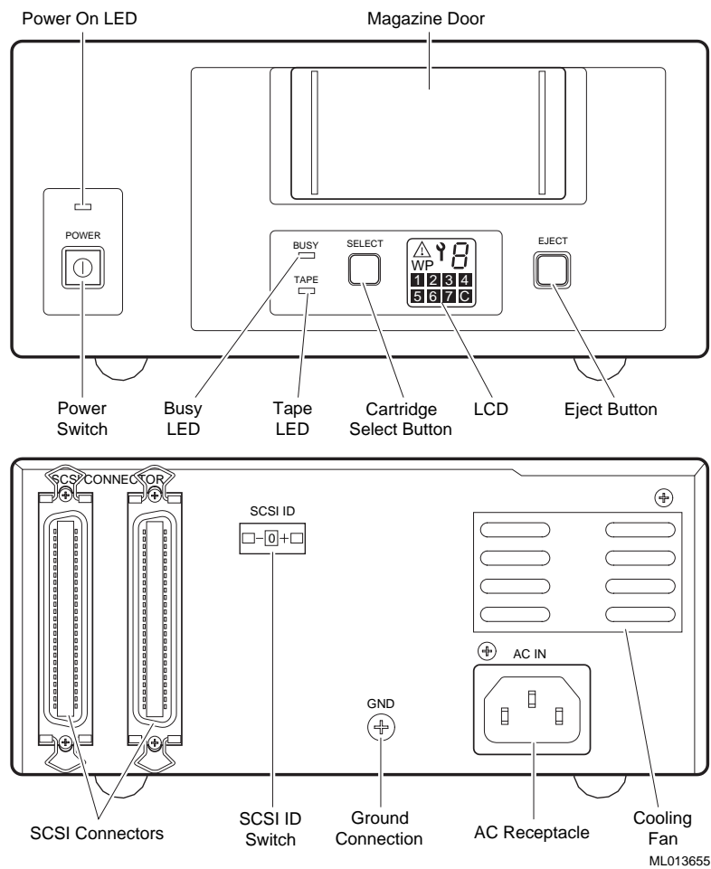
Figure 7-3 Model TLZ9L-DA/DB (Front and Rear View)
