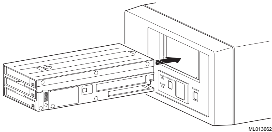
Figure 7-10 Loading the Magazine Into the TLZ9L-DA/DB
