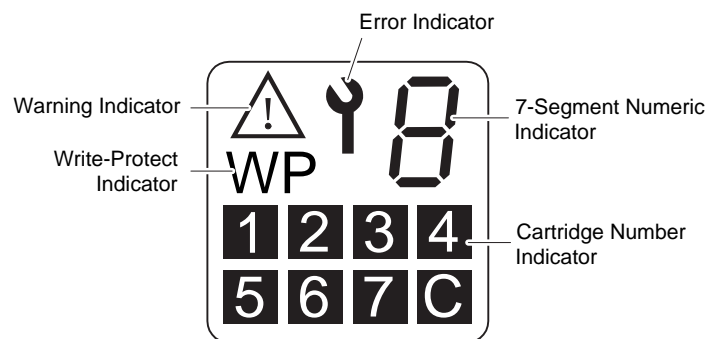
Figure 7-4 TLZ9L LCD Panel
