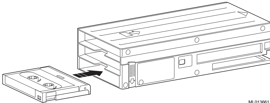
Figure 7-9 Loading Cartridges Into the Magazine
