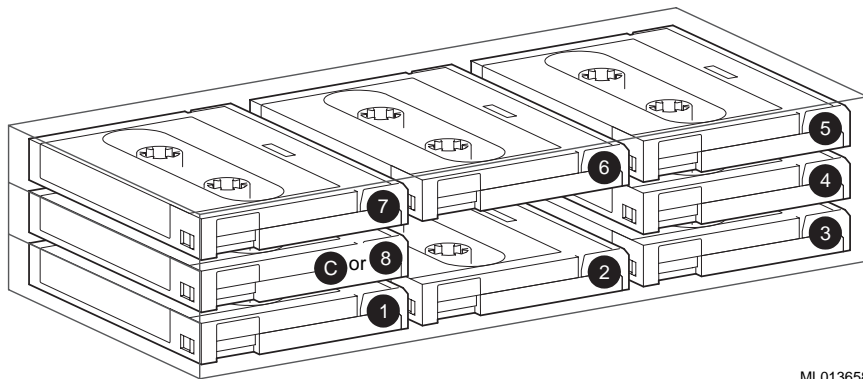
Figure 7-6 Eight Cartridge Mode
