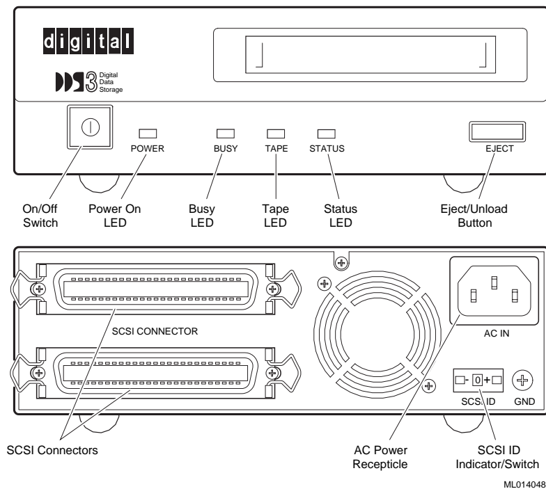
Figure 1-1 Model TLZ09-DA/DB and DS-TLZ10-DB (Tabletop)
