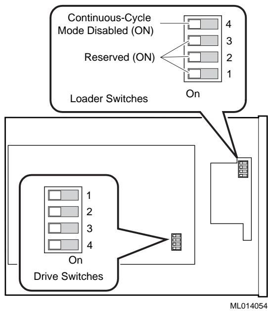
Figure 7-2 Model TLZ9L-AA Bottom View
