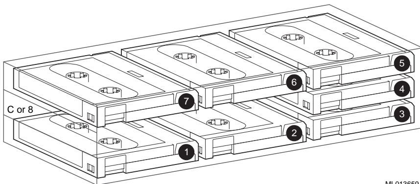
Figure 7-7 Seven Cartridge Mode
